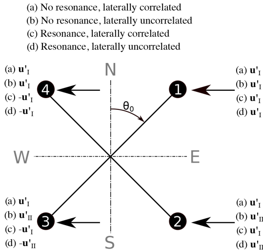
Figure 3. Overview of the assumptions made to determine the cross-contamination values listed in Table 3. In cases with no resonance, the wind vectors u'_{I,II} are identical at the longitudinally separated measurement points. In resonance cases they have an opposite sign. In cases with laterally correlated velocities, the wind vectors at laterally separated measurement points are identical. In cases with no correlation at points that are laterally separated, the wind vectors u'_I and u'_{II} are independent.
