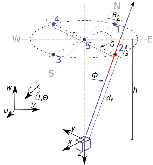
Figure 1. Visualization of the beam configuration of the Windcube V2, relevant lengths and angles, and the two coordinate systems used by the lidar and in wind data analysis. For better visibility, only LOS2 is depicted as a beam, with the range gate indicated in red along the blue laser beam.
