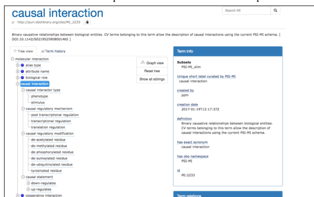
Fig. 2. The hierarchical structure of the new PSI-MI controlled vocabularies terms. Causal Interaction class and child terms as shown in the Ontology Lookup Service (OLS)
