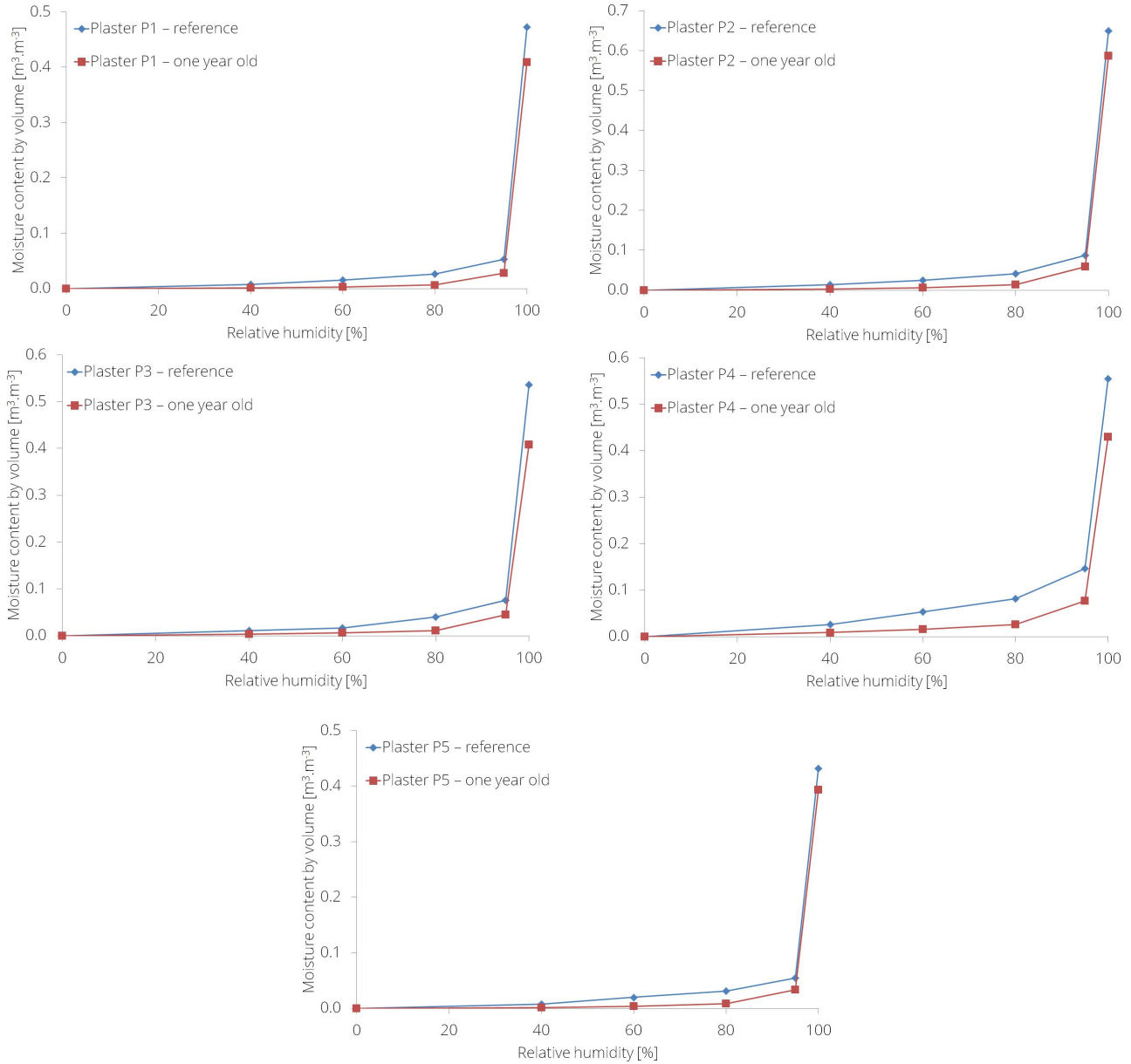
FIGURE 6. Sorption isotherms of studied plasters.
