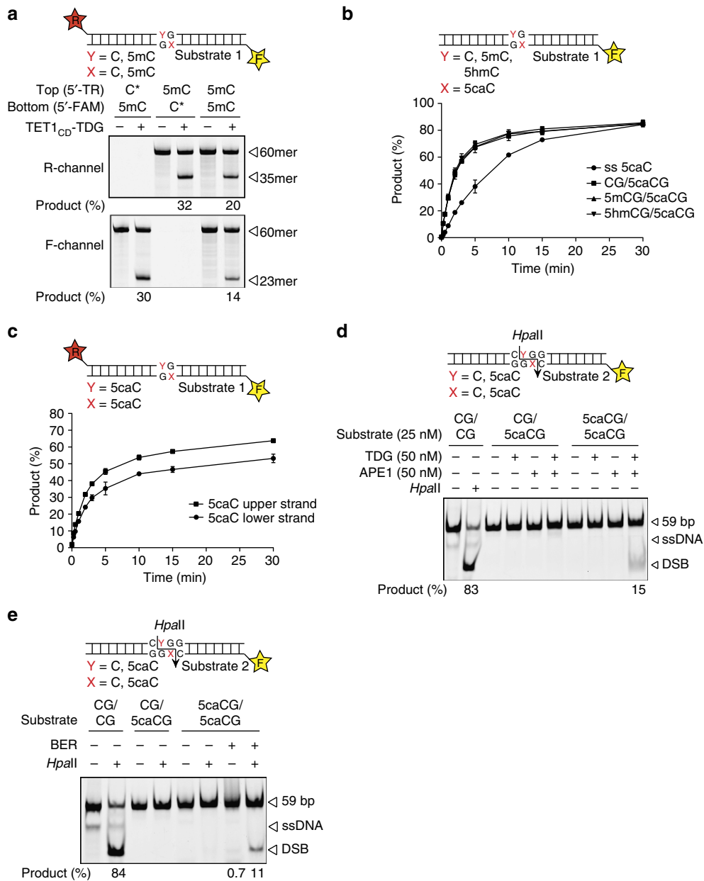
Figure 5 | Processing of differentially modified CpGs by TET1 CD -TDG or TDG. (a) Base release from fully methylated CpGs by His6-TET1 CD -His6-TDG. His6-TET1 CD -His6-TDG (50 nM) was incubated with labelled 60mer substrates (25 nM) containing a single 5mC modification on the fluorescent labelled top (5'-Texas Red, T) or bottom strand (5'-fluorescein, F) or a fully methylated CpG with labels on both strands. Product formation was monitored and quantified by denaturing gel electrophoresis and fluorescent scanning (Texas Red, R-channel and fluorescein, F-channel); positions of the 60mer substrate DNA and the resulting base incision products of both strands are indicated. *Unlabelled DNA strand. (b) Release of 5caC from differentially modified CpGs by His6-TDG. 60mer DNA substrates (25 nM) containing 5caC opposite C, 5mC or 5hmC in a CpG dinucleotide or in single-stranded (ss) DNA were incubated with His6-TDG (25 nM) and analysed by denaturing gel electrophoresis. Shown are mean percentages of product formation with s.d. (n = 3). (c) 5caC release from a symmetrically modified CpG dinucleotide by His6-TDG. A substrate (25 nM) containing 5caC on both strands within a CpG dinucleotide and labels of both strands was incubated with His6-TDG (25 nM) for indicated time, analysed by denaturing gel electrophoresis and visualized by fluorescent scanning of both labels. Shown are mean percentages of product formation with s.d. (n = 3). (d) TDG and APE1 only generate DNA DSBs at symmetrically modified CpGs. Base release assay using TDG and APE1 on a labelled 59-bp substrate containing either a single 5caC or a symmetrically 5caC-modified base pair within a HpaII recognition site (CCGG). Reactions were analysed by native PAGE. Substrate DNA and product fragment are indicated. (e) Full reconstitution of TDG-BER on a symmetrically modified 5caC substrate. A labelled 59-bp substrate (25 nM) containing a symmetrically 5caC-modified base pair within a HpaII recognition site (CCGG) was incubated with TDG (40 nM) and BER factors (200 nM APE1, 40 nM POLβ and 40 nM XRCC1-LIG3). Recovered DNA was digested with HpaII endonuclease and analysed by native PAGE. Substrate DNA and product fragments are indicated; ssDNA, free single-stranded DNA.
