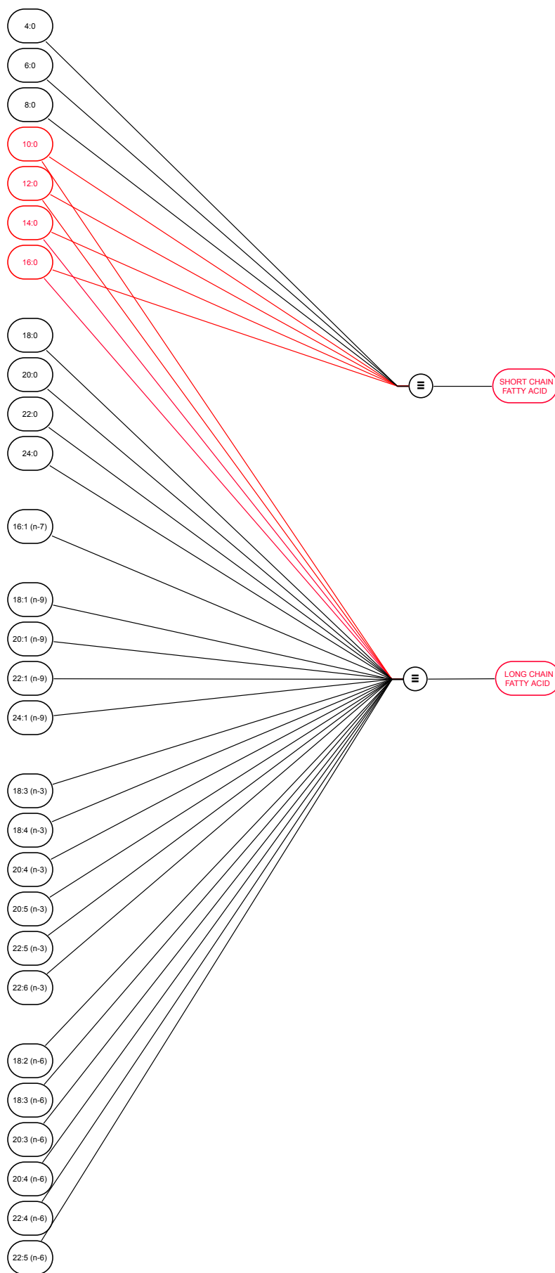
Figure B.3: An example of misuse of the equivalence operator. The use of the equivalence operators does not respect the first rule, because the two generic pools colored in red on the right of the equivalence operator do overlap.
