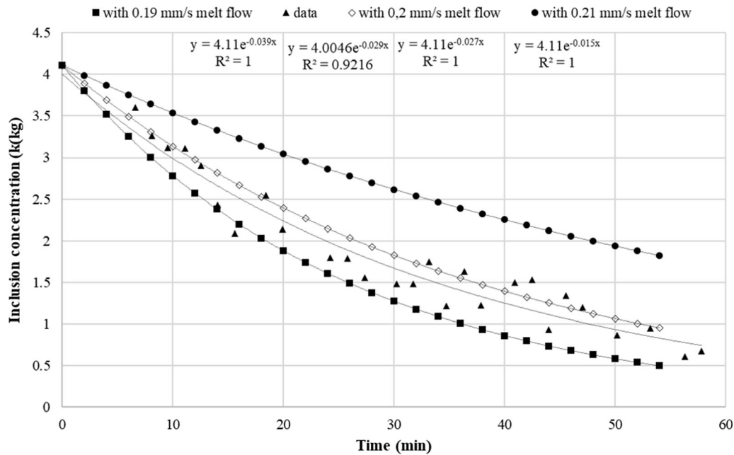
Fig. 11—Settling behavior of discs ( A_R = 50 ) in horizontal orientation under different melt flow velocities in comparison with the LiMCA data.
