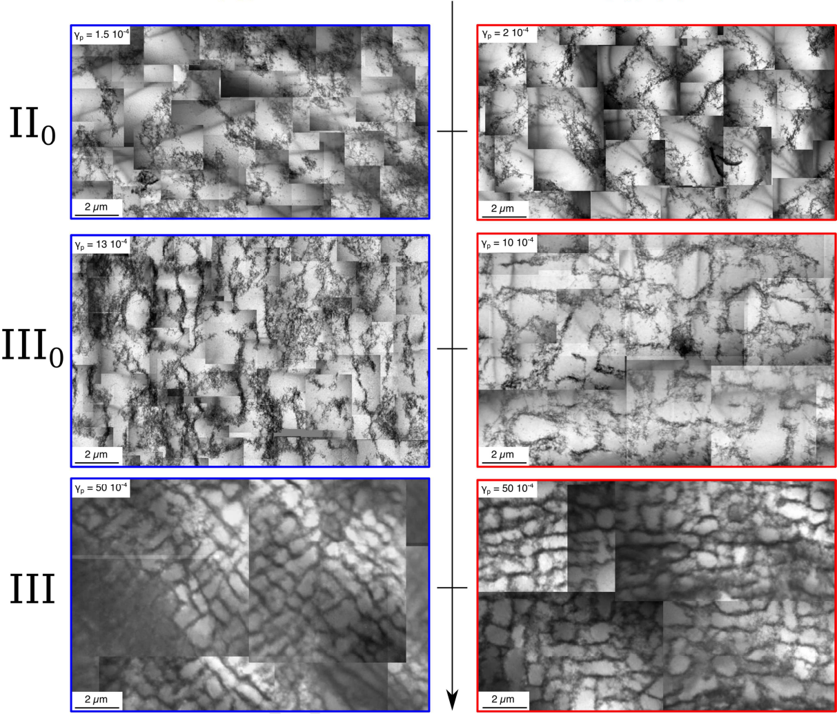
Figure 4: Microstructure induced by cyclically strained nickel (left) and nickel-hydrogen systems (right) at stages II_0 (top), III_0 (middle) and III (bottom).
