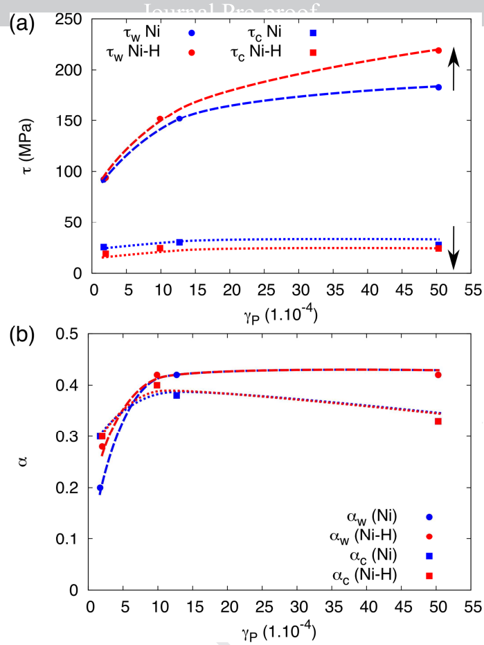
Figure 8: Stress (a) and geometrical \alpha -factor (b) induced by wall and channel phases for the hardening stages II_0 , III_0 and III for pure nickel (blue) and Ni-H systems (red).
