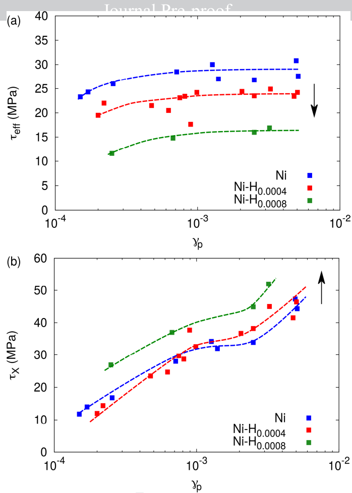
Figure 3: Influence of hydrogen on the effective stress \tau_{eff} (a) and back stress \tau_X (b) of nickel single crystal. The black arrows highlight the effect of the solute on the internal stresses.
