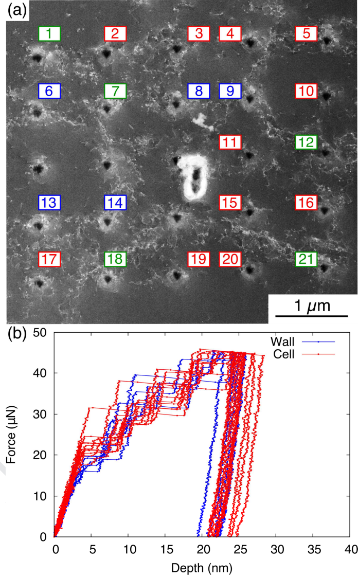
Figure 6: ECCI of indents made on cyclically pre-strained Ni-H systems ( \gamma_p=7.5 \times 10^{-4} ) (a). Corresponding load-displacement curves of indents that are hitting wall or channel phases (b).
