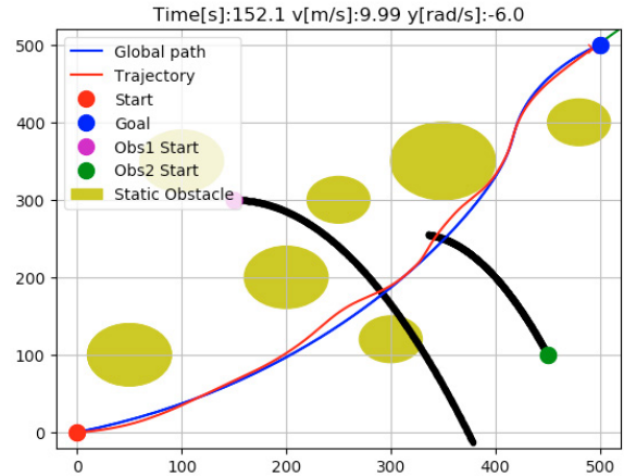
Fig. 4. DW trajectory with circular-arc moving obstacles
