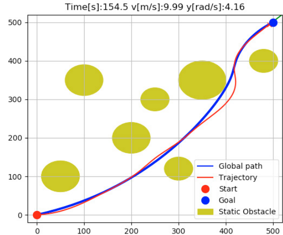
Fig. 1. DW trajectory with static obstacles
