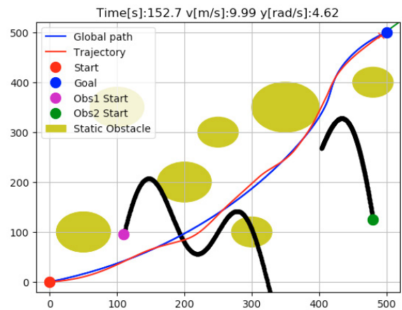
Fig. 5. DW trajectory with random moving obstacles
