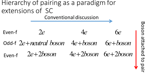
FIG. 5 (Color online) A hierarchy of superconducting states beyond simple pairs is shown. The horizontal axis represents the increased even number of fermions that one condense such as 2e, 4e, 6e condensates. Alternative extensions based on the composite states are shown along the vertical axis. If we start with the conventional paired states, we can extend it to the 2e + 1 boson state. This would correspond to the order parameter as a first derivative of the odd- \omega amplitude and thus this line describes Berezinskii composite pairs. The next step in this process would be a paired state with 2e pair and two bosons that would correspond to second derivative and therefore to even- \omega pairing. The third line would correspond again to the odd- \omega state with three bosons attached to a pair, and so forth.
