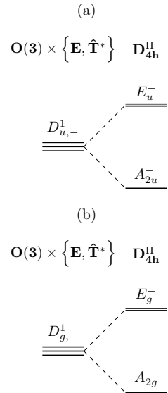
FIG. 2 (Color online) Splitting of pairing states for a pairing potential with D_{4h}^{\text{II}} symmetry. (a) p -wave spin-singlet and (b) s -wave spin-triplet.
