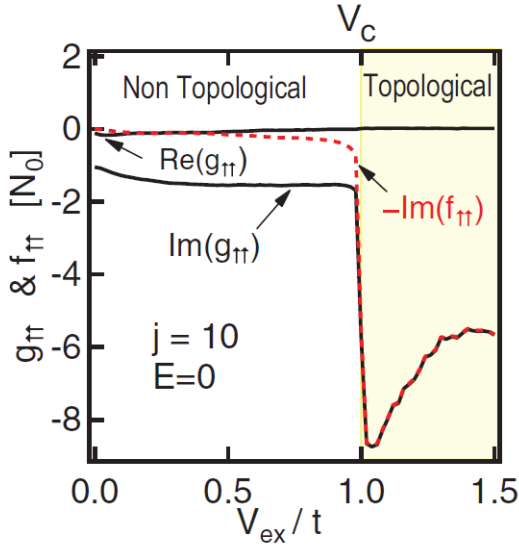
FIG. 27 (Color online) The normal ( g_{\uparrow\uparrow} ) and anomalous ( f_{\uparrow\uparrow} ) Green functions plotted at the superconducting interface (lattice position j = 10 in this model) for E = 0 as a function of the exchange field strength V_{ex} normalized to the hopping amplitude t . At the topological phase transition V_{ex} = V_c where the Majorana fermion emerges, the odd- \omega amplitude has a sharp increase. Figure adapted from (Asano and Tanaka, 2013).
