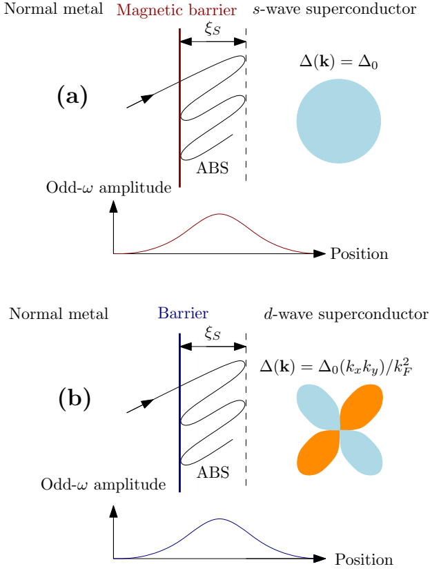
FIG. 22 (Color online) (a) Andreev-bound state (ABS) formed at the interface between a normal metal and s -wave superconductor separated by a magnetic barrier, e.g. a ferromagnetic insulator. The spin-dependent phase-shifts arising due to the magnetic barrier give rise to an interface state which appears at zero-energy for strong enough phase-shifts. (b) ABS formed at the interface between a normal metal and a d -wave superconductor separated by a non-magnetic barrier, e.g. an insulator. The electron- and hole-like excitations experience different signs of the pair potential \Delta(\mathbf{k}) upon scattering, leading to the formation of a zero-energy state. In both (a) and (b) , the bound state at the interface is accompanied by a strong increase in the magnitude of the odd- \omega correlations, quantified via the anomalous Green function f . The dashed line indicates how quasiparticles are Andreev-reflected back toward the interface by the pair potential \Delta(\mathbf{k}) after penetrating a distance \sim \xi_S into the superconductor.
