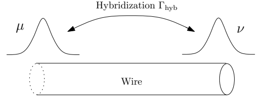
FIG. 24 (Color online) Two Majorana modes localized at the end of a wire with a finite hybridization \Gamma_{\text{hyb}} , as considered in Ref. (Huang et al. , 2015).
