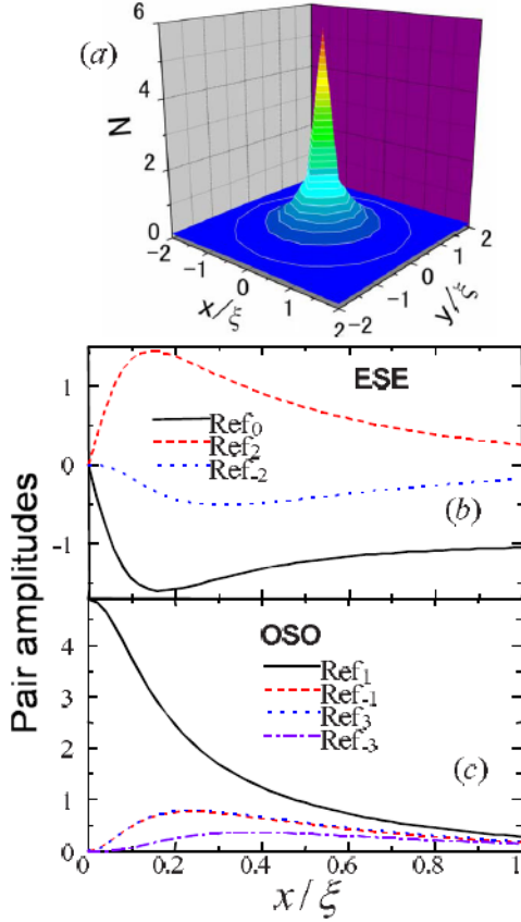
FIG. 10 (Color online) Results for the DOS and Cooper pair symmetry near the vortex core of a conventional s -wave BCS superconductors. (a) Normalized local DOS around the vortex at E = 0 . The center of the vortex is situated at x = y = 0 . Spatial dependencies of (b) even- \omega singlet (ESE) and (c) odd- \omega singlet (OSO) correlations at E = 0 . f_j corresponds to the different angular momentum components of the anomalous Green function f = \sum_n f_n e^{in\theta} , and all have a spin-singlet symmetry. Figure adapted from (Yokoyama et al. , 2008).
