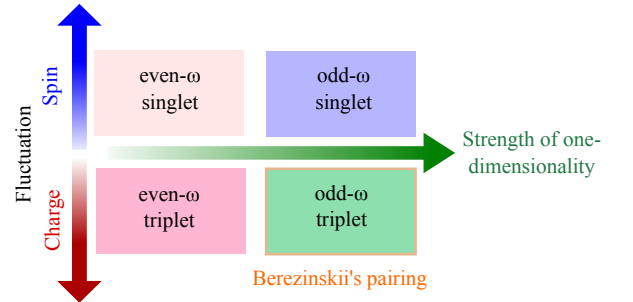
FIG. 13 (Color online) Qualitative dependence of the most stable superconducting pairing symmetries on the degree of one-dimensionality and spin/charge fluctuations. Adapted from (Shigeta et al. , 2011).
