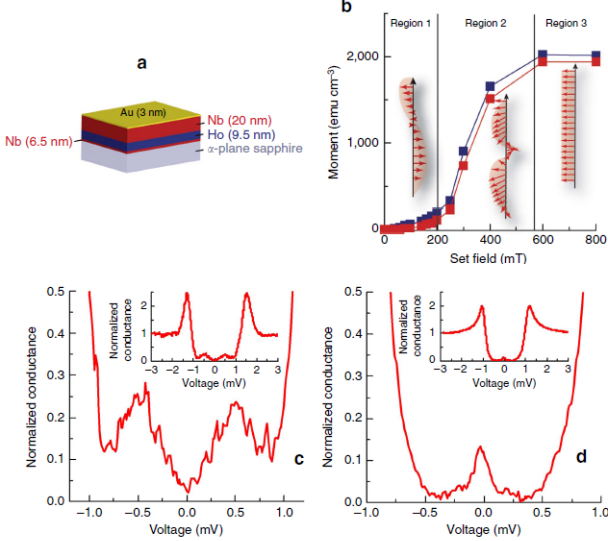
FIG. 18 (Color online) (a) The sample structure on which the STM measurements were performed: an Au/Nb/Ho/Nb multilayer. (b) The magnetization of Ho at zero field (remanent magnetization M_r : red line) and with the set field H switched on (blue line). The vertical (black) lines separate different magnetic phases of Ho: a bulk helix (region 1), coexisting helix and F component (region 2), and F state (region 3). (c) and (d) show typical subgap features obtained in the normalized conductance.
