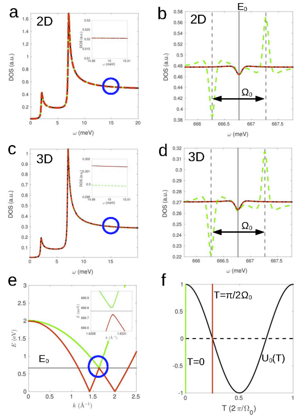
FIG. 8 In (a) and (b), the 2D DOS computed using: effective masses, m_a = 0.5 \text{ \AA}^{-2}/\text{eV} and m_b = 1 \text{ \AA}^{-2}/\text{eV} ; chemical potentials, \mu_a = \mu_b = 2\text{eV} ; s -wave gaps, \Delta_{aa} = 2\text{meV} , \Delta_{bb} = 7\text{meV} , \Delta_{ab} = \Delta_{ba} = 0 , consistent with \text{MgB}_2 (Choi et al. , 2002); interband scattering, \Gamma = 10 \text{ meV} ; dissipation described by \eta = 0.1\text{meV} ; and a drive with U_0 = 10\text{meV} , and \Omega_0 = 1\text{meV} (242 GHz). In both panels we show the case for no drive in black (solid), and the cases with the drive at times T_{\text{cm}} \equiv T = 0 and T = \pi/2\Omega_0 in green (dashed) and red (dash-dotted), respectively. In (a) we focus on the states near the Fermi surface, in (b) we focus on the range of energies near the crossing of the two bands at which we find the driven DOS at T = 0 possesses two peaks shifted from the avoided crossing at E_0 by, \pm\Omega_0/2 . In (c) and (d), the 3D DOS plotted for the same parameters as in (a) and (b). Notice that the main difference is that in 3D the driven DOS at T = 0 is slightly suppressed relative to the undriven DOS (see inset). In (e) we plot the spectrum of the two band superconductor given by \epsilon_{\pm}(\mathbf{k}) . The horizontal grey line denotes the avoided crossing (see inset) at E_0 , due to the finite interband scattering, \Gamma . In (f) we show the drive plotted in the time domain over a full period, the green vertical line denotes the beginning of the period at T = 0 where the drive has maximum amplitude, while the red line denotes T = \pi/2\Omega_0 where the drive amplitude is zero. Adapted from (Triola and Balatsky, 2016).
