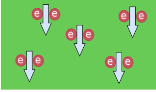
Odd- \omega pairing: Composite Cooper pair + boson (spin/lattice)
