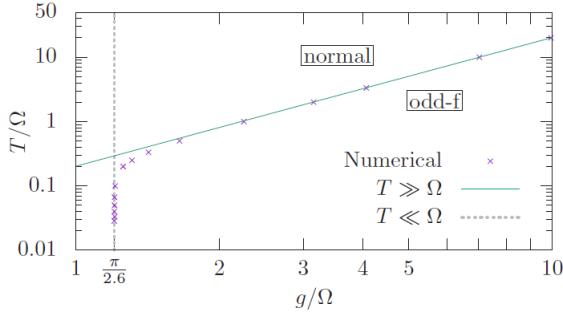
FIG. 26 (Color online) Phase diagram of the normal and pairing state of collection of Majorana states is shown. For the large coupling between the ends of the wire, the system will have a strong pairing fluctuations in the odd- \omega channel. The phase diagram is drawn for the mean field solution of the pairing state. As explained, Majorana states have a strong propensity to form the odd- \omega state. The green solid line shows the critical temperature T_c \propto g^2 . From Ref. (Huang et al. , 2015).
