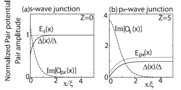
FIG. 14 (Color online) Spatial dependence of the pair potential normalized against its bulk (solid line) and the even- \omega spin-singlet pair amplitudes E_s(x) ( s -wave channel) and E_{p_x}(x) ( p -wave channel) for an SN ballistic bilayer. The x -axis extends into the superconducting layer. The odd- \omega pair amplitudes in the corresponding angular momentum channels are denoted O_s(x) and O_{p_x}(x) . The parameter Z quantifies the junction transparency, with Z = 0 corresponding to a perfect interface and Z \gg 1 corresponding to the tunneling limit. In (a), the superconductor is of the conventional s -wave BCS type whereas in (b) the superconductor is of the p x type. The ballistic superconducting coherence length is \xi = v_F/\Delta . Figure adapted from (Tanaka et al. , 2007b).
