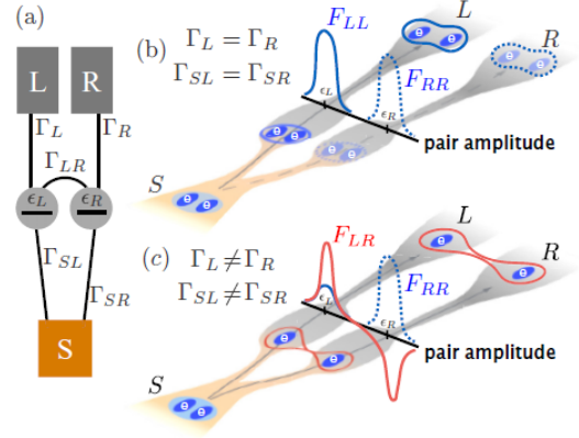
FIG. 21 (Color online) Suggested experimental setup for electrically controlled odd- \omega pairing in a double-dot three-terminal device. (a) The quantum dots have level positions \varepsilon_{L,R} and are contacted by a superconducting lead S and two normal leads L and R. (b) Illustration of a local Andreev reflection process where the Cooper pair electrons tunnel into a normal lead through one dot. (c) Non-local Andreev reflection (AR) where the two electrons comprising the Cooper pair tunnel into different leads. The blue lines refer to the pair amplitudes F_{LL} and F_{RR} in the case of local AR whereas the red lines illustrate the non-local amplitude F_{LR} which is odd- \omega on the resonance point \varepsilon_L = \varepsilon_R . Figure adapted from (Burset et al. , 2016).
