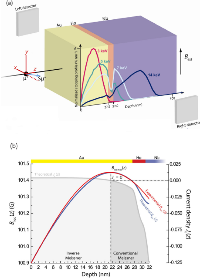
FIG. 19 (Color online) (a) Setup used for observation of the paramagnetic Meissner effect due to odd- \omega -triplets in Ref. (Di Bernardo et al. , 2015b): an Au/Ho/Nb trilayer exposed to an external field B . Low-energy muons injected in Au provided information about the local magnetization profile. (b) Experimental measurement and theoretical fit to the local magnetization signal B_{\text{loc}} as well as the theoretically computed spatial distribution of the shielding current density J_x throughout the system.
