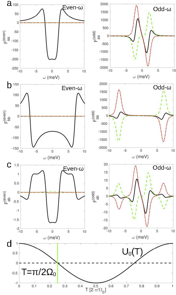
FIG. 7 In the left (right) column we plot the even- \omega (odd- \omega ) terms of the real part of the Wigner transform of the anomalous part of the Green function, \langle \hat{F}^R(\omega, T = \pi/2\Omega_0) \rangle , in black (solid), where we have taken the average value of \hat{F}^R(\mathbf{k}; \omega, T = \pi/2\Omega_0) at |\mathbf{k}| = k_F^{(a)} and |\mathbf{k}| = k_F^{(b)} . In each case we have also plotted the parity-preserving terms (green-dashed) and parity-reversing terms (red-dash-dotted). (a) the diagonal component for band- a , (b) the diagonal component for band- b , (c) the interband component. (d) The components of the drive, plotted in the time domain over a full period, the green vertical line denotes the time, T_{\text{cm}} \equiv T = \pi/2\Omega_0 , at which all plots in this figure are evaluated. The parameters used to describe the driven multiband superconductor in this case are: effective masses, m_a = 0.5 \text{ \AA}^{-2}/\text{eV} and m_b = 1 \text{ \AA}^{-2}/\text{eV} ; chemical potentials, \mu_a = \mu_b = 2\text{eV} ; s -wave gaps, \Delta_{aa} = 2\text{meV} , \Delta_{bb} = 7\text{meV} , \Delta_{ab} = \Delta_{ba} = 0 , consistent with \text{MgB}_2 (Choi et al. , 2002); interband scattering, \Gamma = 10 \text{ meV} ; dissipation described by \eta = 1\text{meV} ; and a drive U(t) = U_0 \cos(\Omega_0 t) with U_0 = 10\text{meV} , and \Omega_0 = 1\text{meV} (242 GHz). Adapted from (Triola and Balatsky, 2016).
