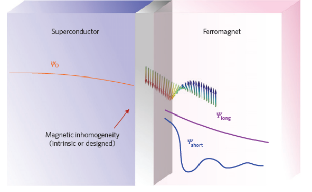
FIG. 17 (Color online) Starting out with a conventional s -wave even- \omega superconductor described by a wavefunction \Psi_0 , a proximity-coupling to a homogeneous diffusive ferromagnet creates short-ranged odd- \omega Cooper pairs with a wavefunction \Psi_{\text{short}} . These rapidly decay in an oscillatory manner inside the magnetic region. In the presence of a magnetic inhomogeneity at the interface, long-ranged odd- \omega Cooper pairs \Psi_{\text{long}} which are spin-polarized (triplet) emerge which penetrate a much longer distance compared to \Psi_{\text{short}} . Figure adapted from (Linder and Robinson, 2015b).
