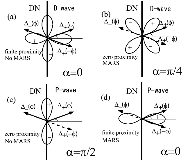
FIG. 15 (Color online) The arrows illustrate the trajectories of scattered quasiparticles at the interface between a diffusive normal metal and an unconventional superconductor with a d -wave symmetry [(a) and (b)] and a p -wave symmetry [(c) and (d)]. The angle \alpha denotes the angle between the normal to the interface and the crystal axis in the d -wave case and the lobe direction in the p -wave case. The angle \phi denotes the injection angle of quasiparticles as measured from the x -axis. Figure adapted from (Yokoyama et al. , 2005).
