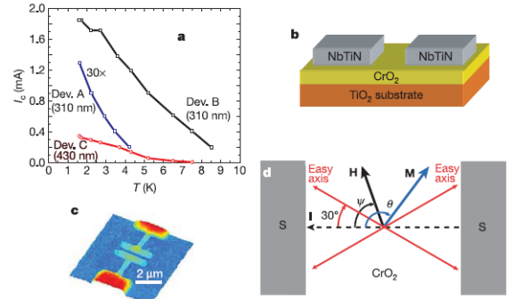
FIG. 16 (Color online) (a) Critical supercurrent as a function of temperature for different separation distances between the superconducting electrodes. (b) Schematic setup of the studied devices, consisting of a lateral Josephson junction with two superconducting electrodes deposited on the half-metal CrO 2 . (c) Scanning electron micrograph of a typical final device. (d) Illustration of the alignment of the current direction with respect to the magnetization axes: I is the current, H is the applied magnetic field, and M is the magnetization. Figure adapted from (Keizer et al. , 2006).
