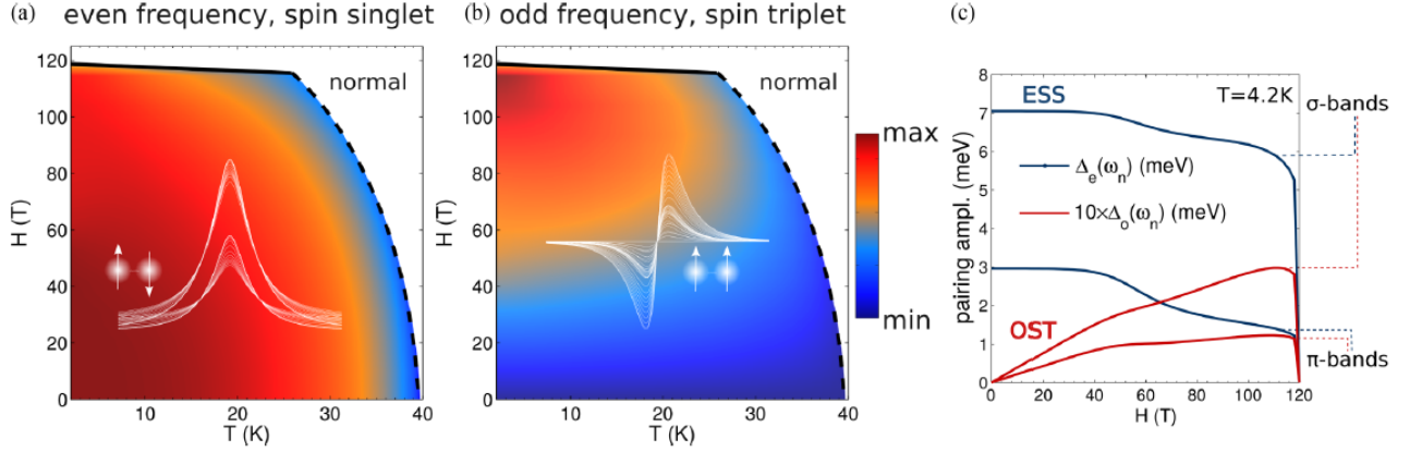
FIG. 11 (Color online) (a) The H - T_{\text{temp}} phase diagram for the even- \omega superconducting order parameter in MgB 2 . Dashed (solid) lines indicate a second (first) order phase transition. (b) H - T_{\text{temp}} phase diagram for the odd- \omega superconducting order parameter. The insets in both (a) and (b) show the Matsubara frequency dependence of the order parameters for different magnetic field values. The color bar max/min values are 7 meV/0 meV for the even- \omega amplitude and 0.3/0.0 meV for the odd- \omega amplitude. (c) The band-resolved field dependence of the even- \omega and odd- \omega order parameters at low temperature. The lines correspond to the maximum values in Matsubara space of the momentum averaged superconducting order parameters on each band, which is equivalent to the peaks in the insets of (a) and (b). Adapted from (Aperis et al. , 2015).
