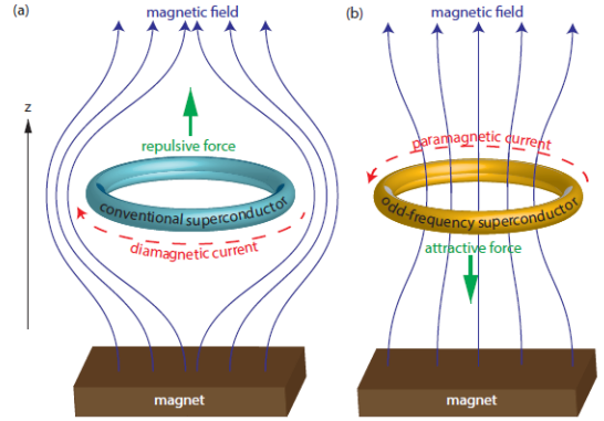
FIG. 9 (Color online) Meissner responses of (a) a conventional superconducting ring and (b) an odd- \omega superconducting ring. In the event of a paramagnetic supercurrent response, the odd- \omega superconductor experiences an attractive force to the underlying magnet, causing superconducting antilevitation. Figure adapted from (Lee et al. , 2016).
