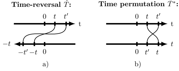
FIG. 1 (a) Time-reversal \hat{T} and (b) time-permutation \hat{T}^* symmetries for two times; an odd-frequency superconductor breaks the time-permutation symmetry \hat{T}^* .
