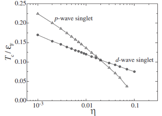
FIG. 3 (Color online) Transition temperature T_c for p - and d -wave spin-singlet pairing as a function of \eta . Figure adapted from (Fuseya et al. , 2003).
