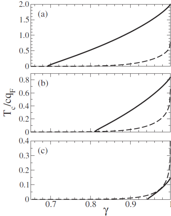
FIG. 29 (Color online) Critical temperature T_c vs. the scaled fermion-phonon coupling \gamma . Solid line: critical temperature for s -wave odd- \omega pairing. Dashed line: critical temperature for p -wave pairing. We have defined c_S as the phonon speed of sound and \xi = \sqrt{\xi_0^2 + \gamma/12q_F^2} where \xi_0 is the boson coherence length. Figure adapted from (Kalas et al. , 2008).
