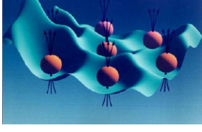
QHE: Composite state of fermion + boson (flux tubes)
