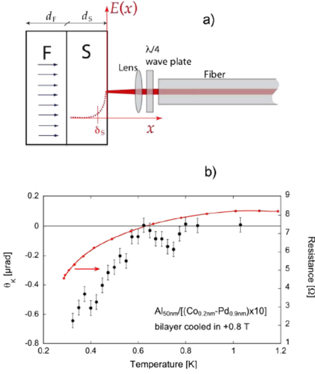
FIG. 20 (Color online) (a) Schematic measurement setup used in (Xia et al. , 2009): two perpendicularly linearly polarized lights emerging from the fiber become circularly polarized and focus on the sample using a lens. The electric field E penetrates a short distance \ll d_S into the superconductor. (b) Kerr effect measurement of an Al/(Co-Pd) bilayer system with a 50 nm Al-sample. Figure adapted from (Xia et al. , 2009).
