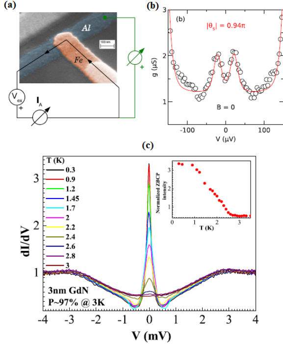
FIG. 23 (Color online) (a) Scanning electron microscopy image of the Al/AlO x /Fe sample used in (Hübler et al. , 2012) along with the measurement scheme. (b) Differential conductance spectrum for the structure at zero magnetic field ( B = 0 ), together with a theoretical fit (red line). (c) Differential conductance ( dI/dV ) measurements (Pal et al. , 2017) normalized to the normal-state value of a 100 nm NbN/3 nm GdN/30 nm TiN tunnel junction demonstrating the evolution of a zero-energy peak with decreasing temperature. Figures (a) and (b) adapted from (Hübler et al. , 2012) and Figure (c) adapted from (Pal et al. , 2017).
