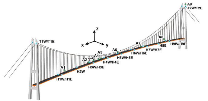
Fig. 3. Positions of the sensors on the Hardanger bridge.
