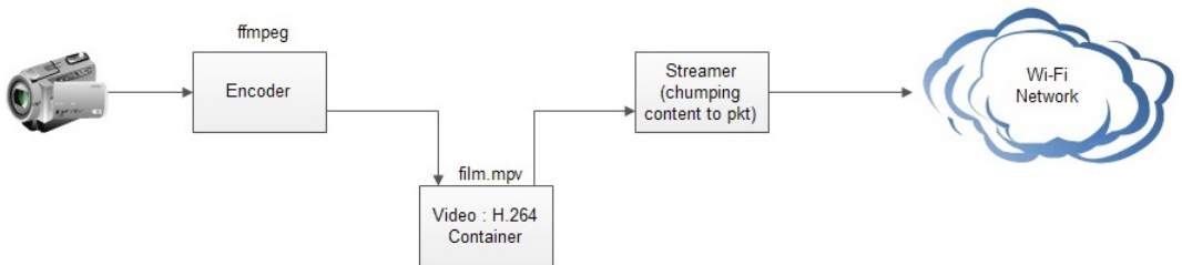
Figure 4.2: Encoding architecture
