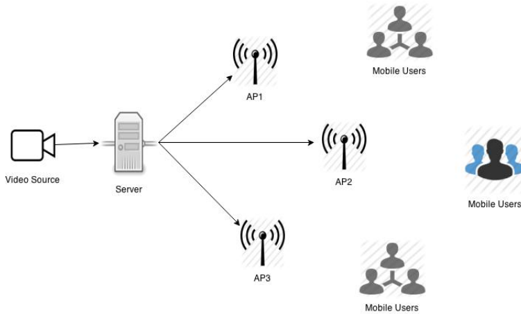
Figure 4.1: Network model
