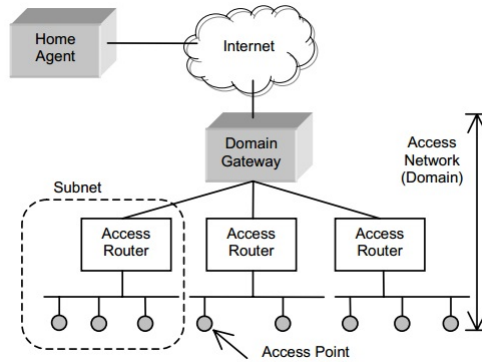
Figure 2.14: micromobility architecture.[28]
