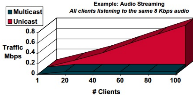
Figure 2.1: Multicast VS Unicast traffic from cisco.com
