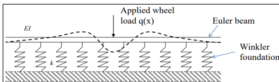
Figure 2.14 - Principle sketch: The main principles behind Zimmermanns theory, a continuously welded rail (CWR) as an Euler-bernullis beam founded on a winkler springbed
