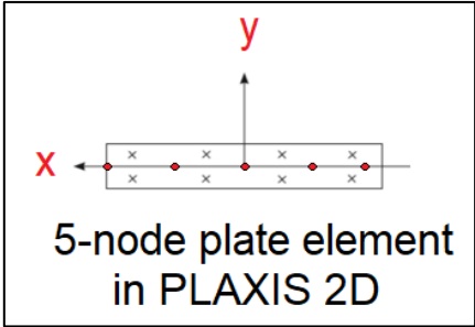
Figure 2.5 – A 5-node plate element in PLAXIS 2D pr. effective meter plate pr. effective meter plane. The axis system corresponds to the same axis system in figure 2.1
