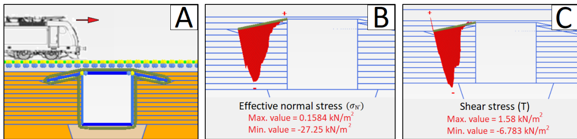
Figure 4.7 – Slab behaviour of the 2.5 meter case, showing A) train location, B) effective normal stress and C) shear stress
