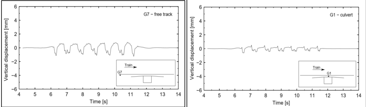
Figure 4.11 – Measurements at the transition zone of Gouda Goverwelle, showing results from the free track and above culvert (Modified after Coelho, B, 2011)
