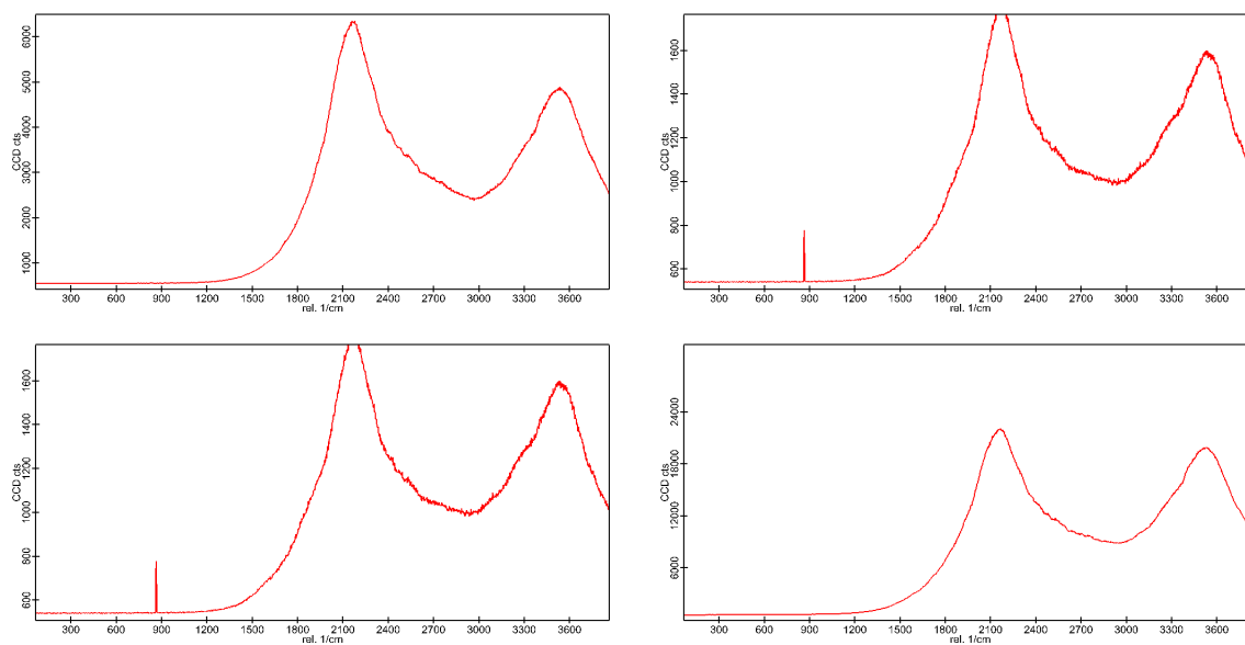
Figure C.2.5: LDPE blue in water
