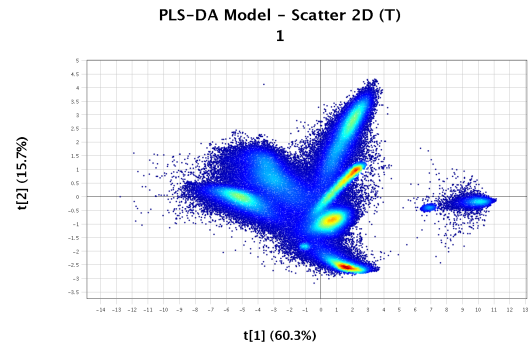
(b) PLS-DA Scatter plot
