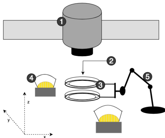
Fig. 3: Laboratory set-up. 1 is the Norsk Elektro Optikk (NEO) SWIR-320m-e imaging spectrometer. 2 is the sample (or the water) placed in the petri dish. 3 is the petri dish of fused silica. 4 is the hypspec infrared halogen light source. 5 is the arm holding the petri dishes with samples and water
