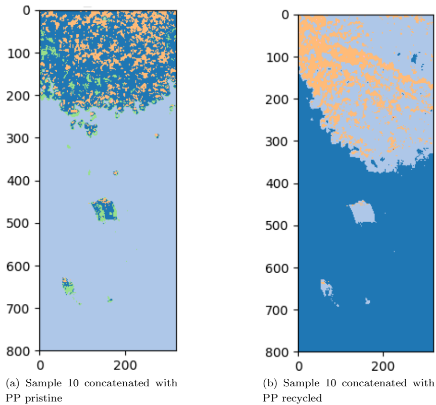
Figure 8.2.6: Revised results from the K-means clustering on the Lofoten samples concatenated with plastic types after reviewing the results from Raman spectroscopy
