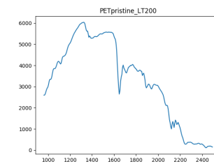
(b) PET Pristine, Smaller than 200 microns
