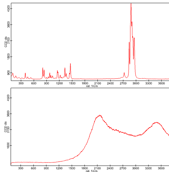
Figure 9.2.6: PP pristine (top), PP recycled (bottom)
