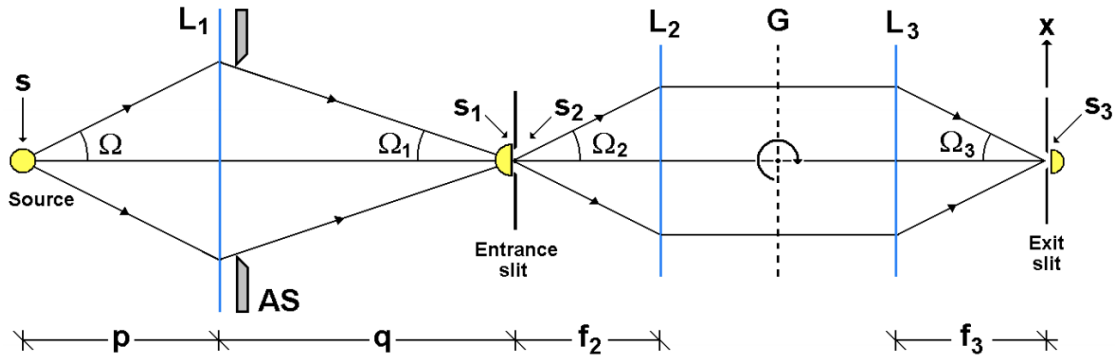
Figure 4.3.1: Optical diagram of a Spectrometer
