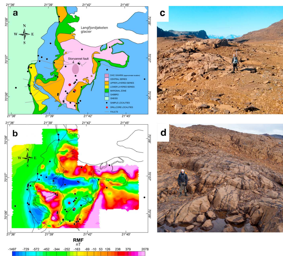
Figure 2. (a) Geological map of the Reinjford Ultramafic complex (modified after Larsen et al., 2018). The sampling locations are indicated in black dots, and drill core locations are indicated by the red circles. Faults are indicated in gray (from Emblin, 1985). The shaded area in the center indicates the approximate location of a dike swarm where the density of dikes is higher than in the rest of the central series (CS). (b) High-resolution helicopter aeromagnetic map (SkyTEM surveys, 2011) showing the residual total magnetic intensity. The outlines of the contacts are shown in black, as well as the sample locations. Field images of the RUC show the superb exposure in the area of the (c) CS and (d) pyroxenite dikes.
