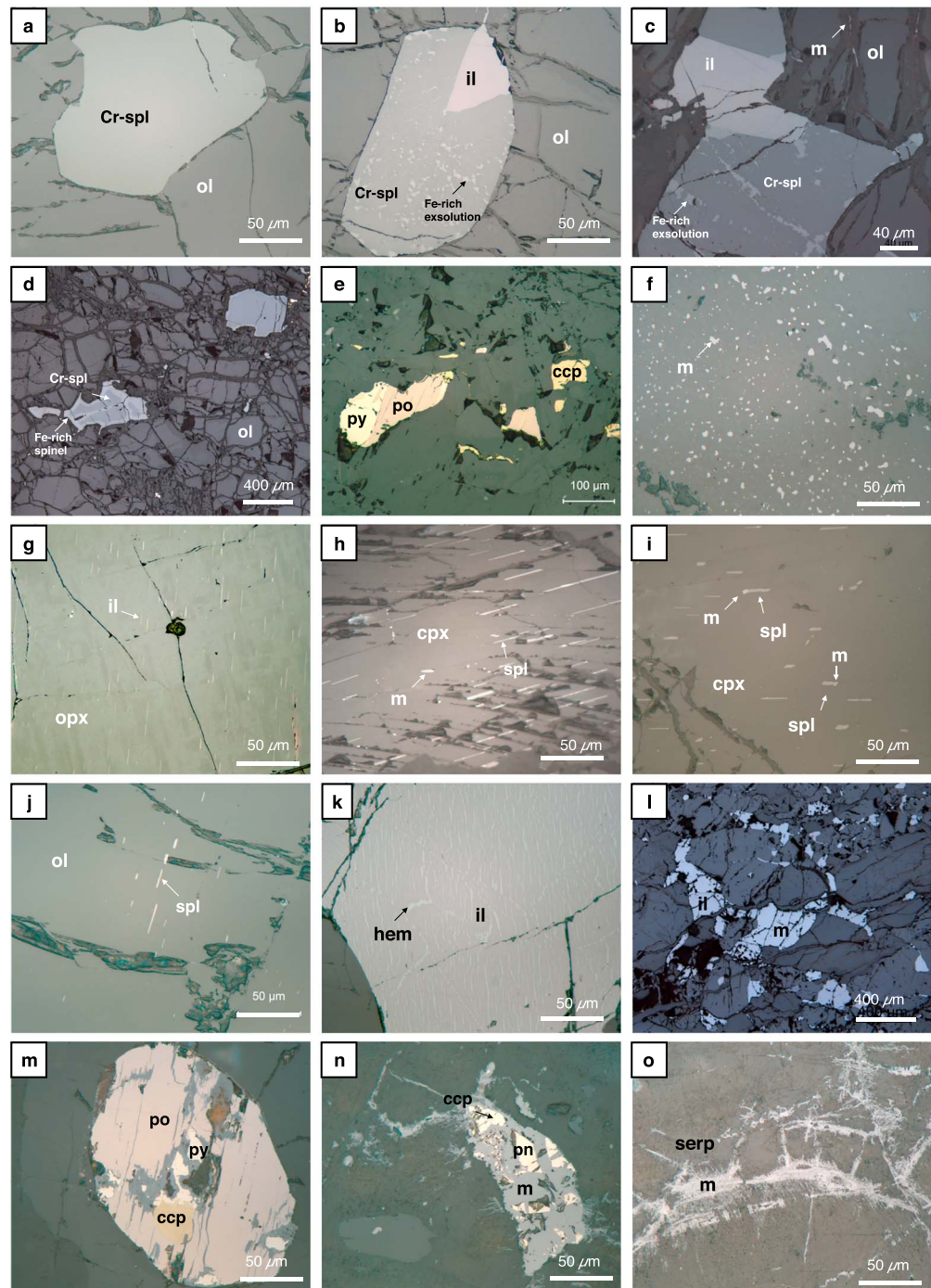
Figure 4. Reflected light images of (a) homogenous chrome-spinel and (b and c) chrome-spinel and ilmenite from central series (CS) surface rocks. The chrome-spinel contains exsolution microstructures of a more iron-rich phase. (d) Chrome-spinel with an iron-rich rim from CS drill core samples. (e) Pyrite, pyrrhotite, and chalcopyrite in the CS surface samples. (f) Magnetite in a pyroxenite dike sample. (g) Exsolution of ilmenite lamellae from orthopyroxene in MZ_gneiss rocks. Exsolution of magnetite and spinel from clinopyroxene in (h) upper layered series (ULS) and (i) MZ_gabbro rocks. (j) Spinel exsolution from olivine in CS rocks. (k) Hemo-ilmenite in gabbro rocks, (l) magnetite, (l) magnetite, and ilmenite in gabbro rocks. (m) Pyrrhotite-chalcopyrite-pyrite in gabbro rocks. (n) Pentlandite-chalcopyrite-magnetite, and ilmenite in CS serpentinite. (o) Magnetite in serpentinite veins in CS serpentinite. m: magnetite; il: ilmenite; hem: hematite; po: pyrrhotite; py: pyrite; ccp: chalcopyrite; Cr-spl: chrome-spinel; spl: spinel; pn: pentlandite; serp: serpentinite.
