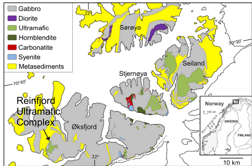
Figure 1. Map of the Seiland Igneous Province in northern Norway modified after Larsen et al. (2018). The ultramafic complexes are indicated in green. This paper focuses on the Reinffjord Ultramafic Complex, which formed adjacent to gabbro and meta-sedimentary gneiss.
