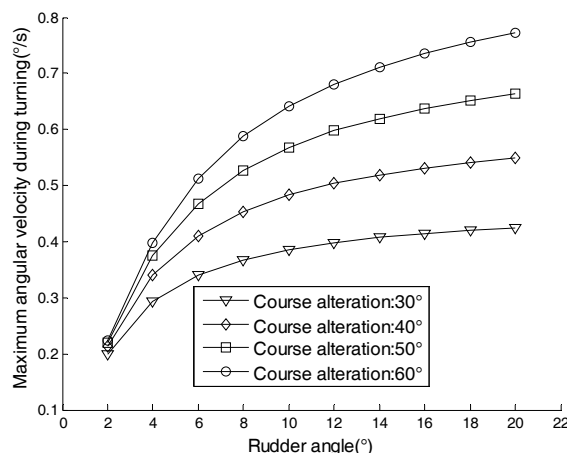
Figure 5. Relationship between rudder angle and the maximum angular velocity during course alteration
