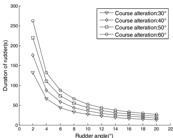
Figure 3. Relationship between rudder angle and the duration for the rudder to keep for course alteration
