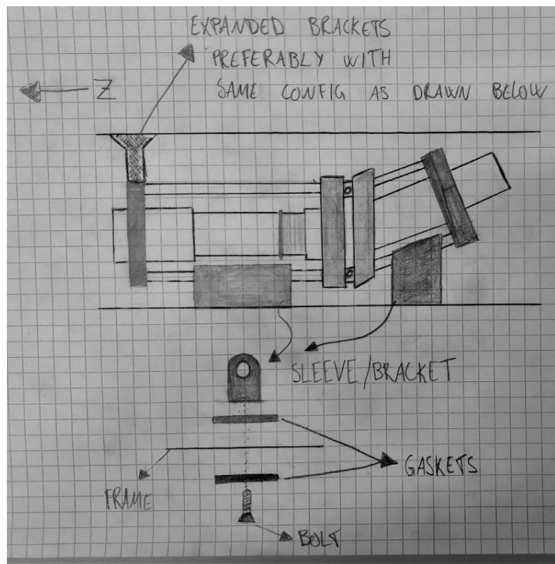
Figure 1: Integrated Bracket Mounting Concept
