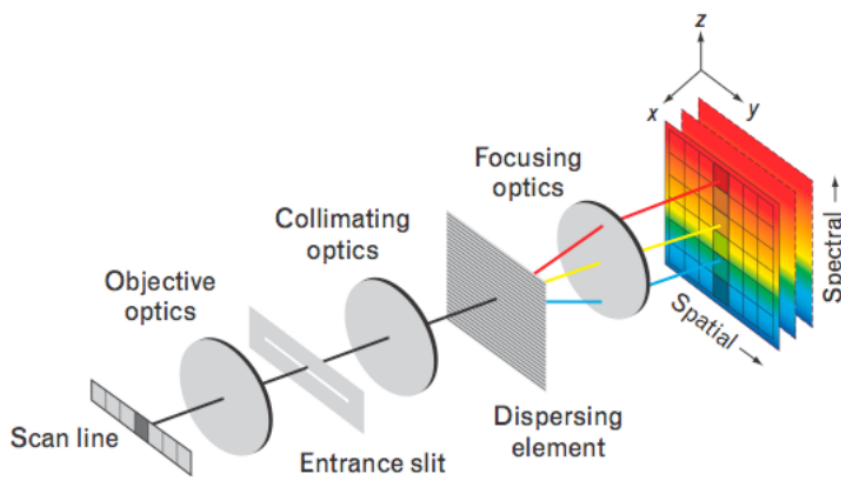
Figure 6: Optical architecture of a Pushbroom HSI
