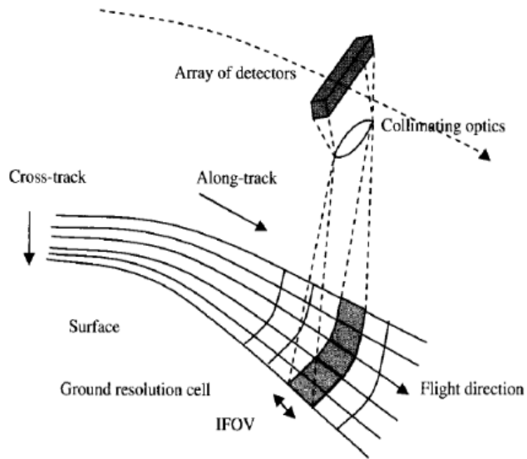
Figure 5: Pushbroom HSI operating on a satellite
