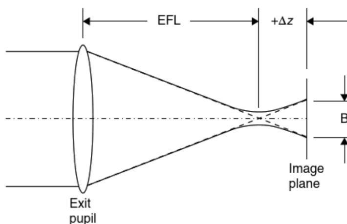
Figure 12: Diagram of Optical misalignment
