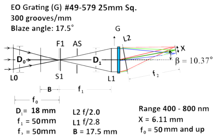
Figure 7: HSI V6 Optical Design
