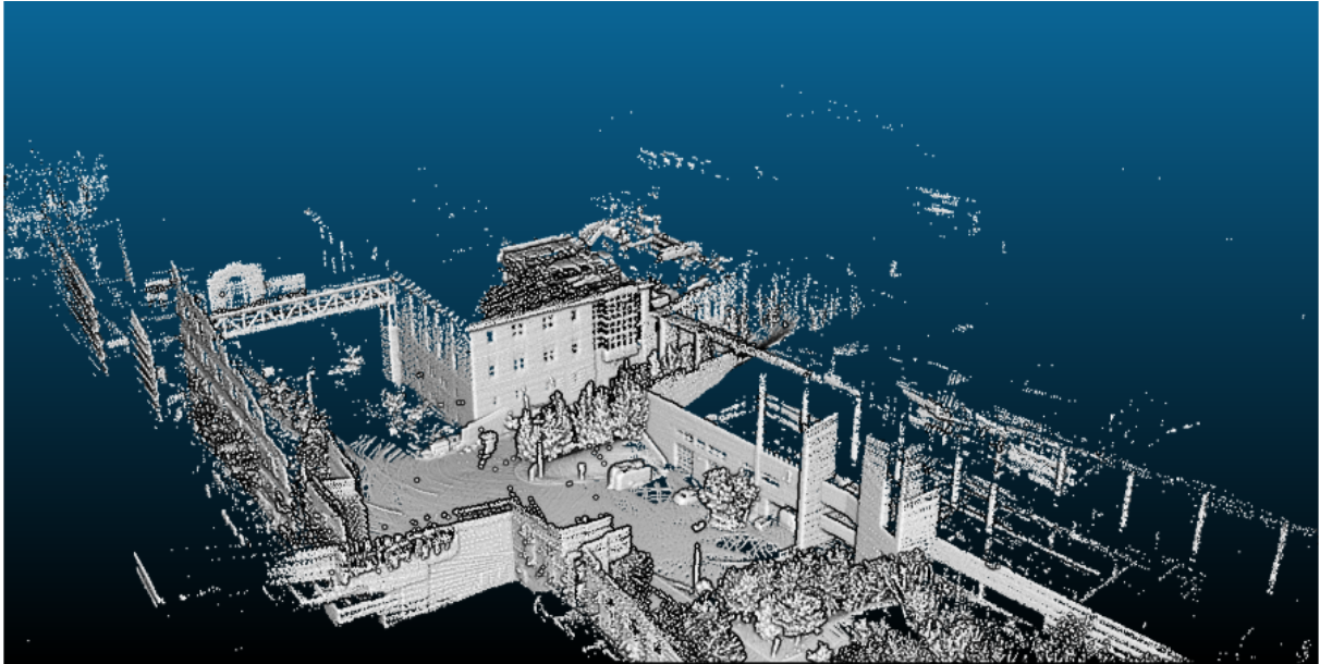
Figure 3.4: Example of map built by LOAM. Courtesy of [59].
