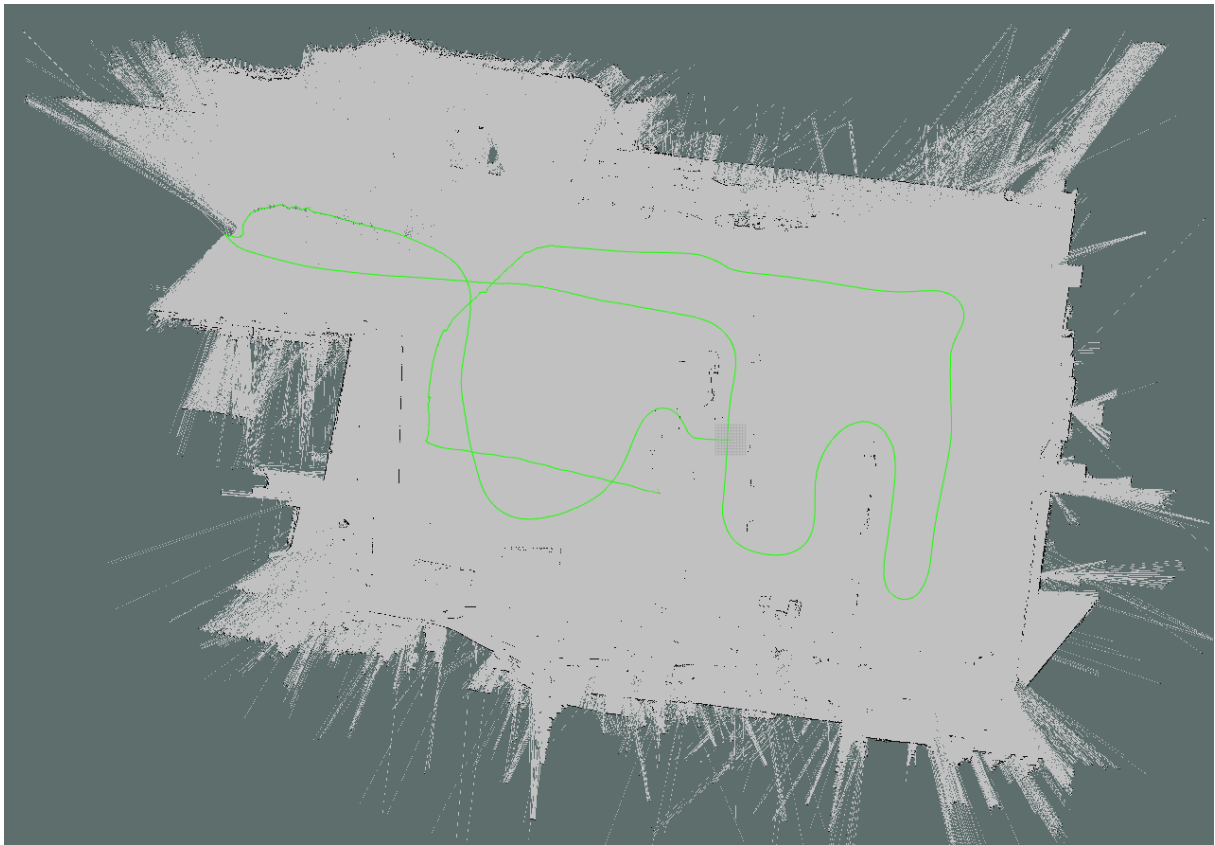
Figure 6.3: Resulting map and trajectory from running Hector-SLAM on the full data-set. Scans were filtered through the laser filter beforehand to get rid of rays hitting MilliAmpere.
