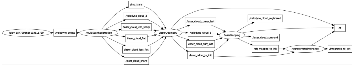
Figure 5.2: ROS-graph when running LOAM on a rosbag, without any filters used. The oval boxes are executable nodes, while the square boxes are topics.
