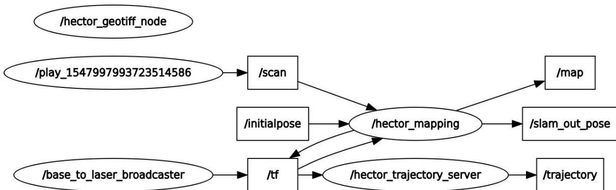
Figure 5.1: ROS-graph when running Hector-SLAM on a rosbag, without any filters used. The oval boxes are executable nodes, while the square boxes are topics.
