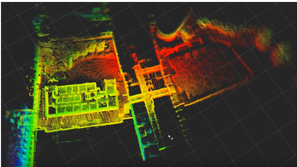
Figure 3.5: Screenshot of map built by BLAM using a Velodyne VLP-16 lidar, placed on top a mans head while traversing a building. Courtesy of [54].
