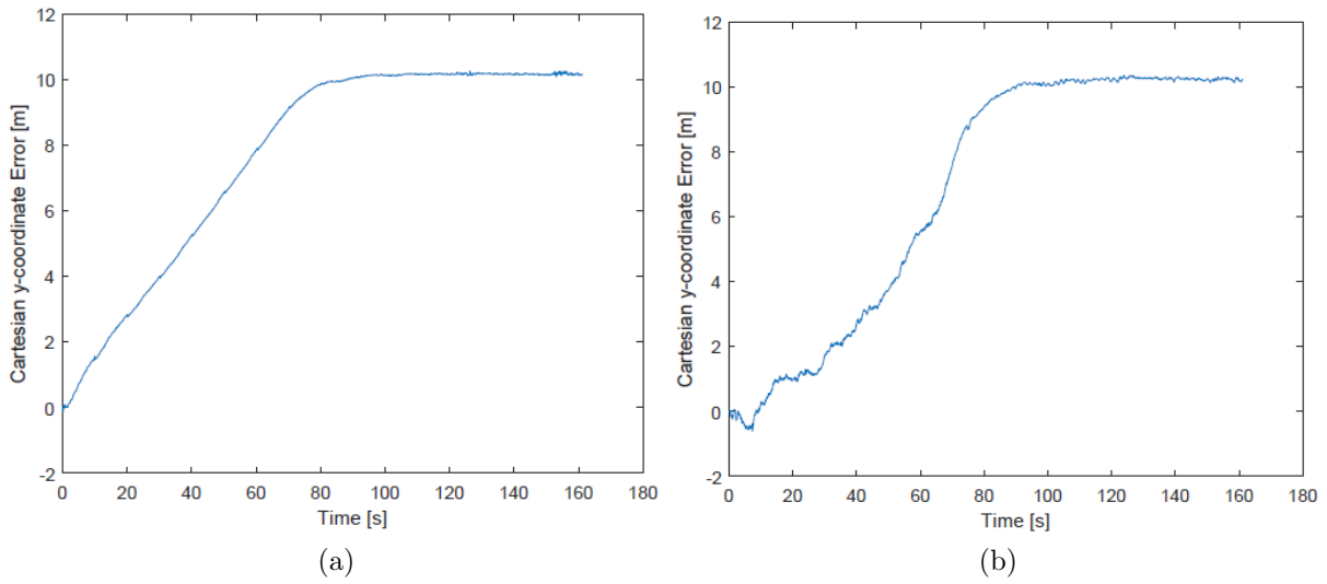
Figure 6.13: (a) shows the error on y for regular HECTOR-SLAM run on the last 161 seconds. (b) shows the error in y for HECTOR-SLAM run on down-projected scans from the last 161 seconds.
