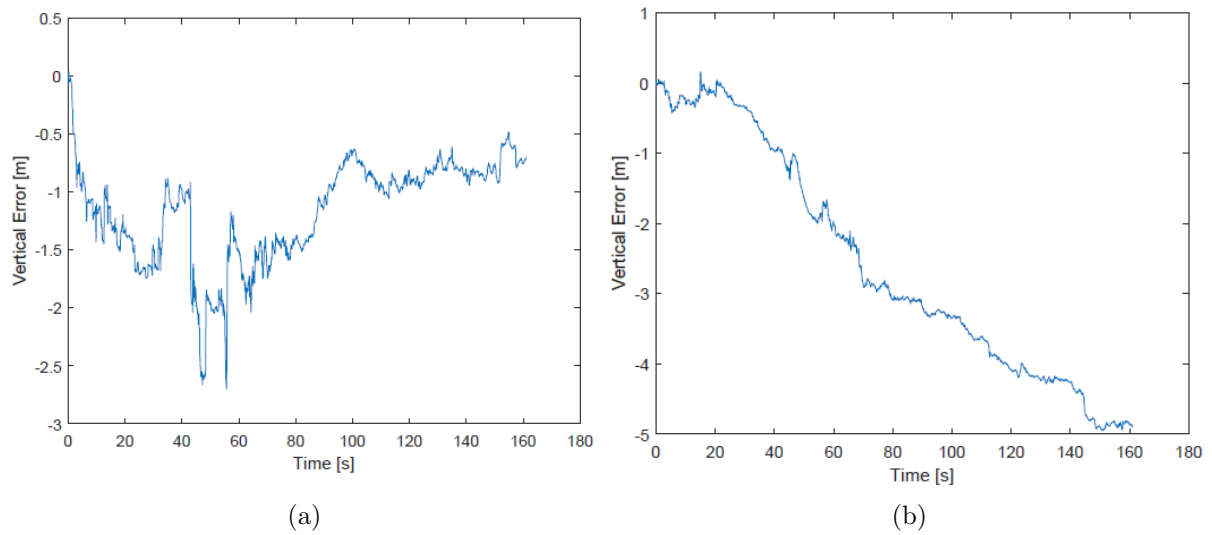
Figure 16: (a) shows vertical drift from BLAM run on the small sized data-set with point cloud filter. (b) shows vertical drift from BLAM run on the small data-set without point cloud filter.
