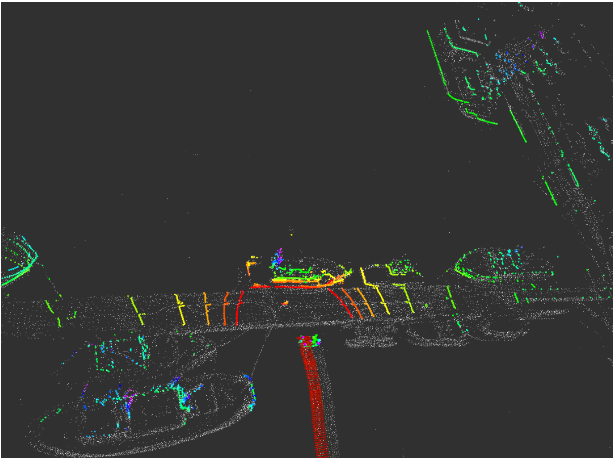
Figure 6.18: Close-up of the LOAMs mapping of the dock, as the map building of the small set is finished.
