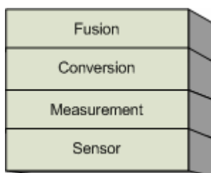
Figure 4: Context stack
