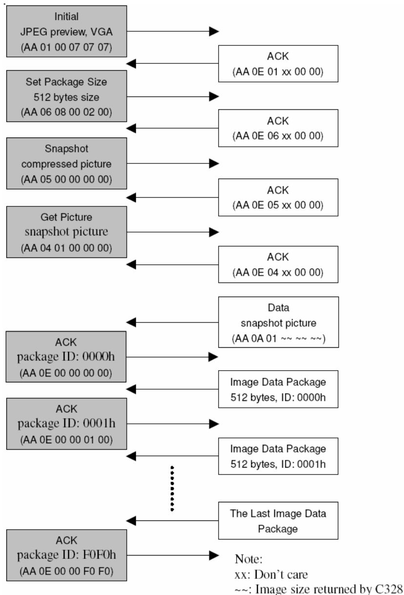
Figure 39: Camera commands
