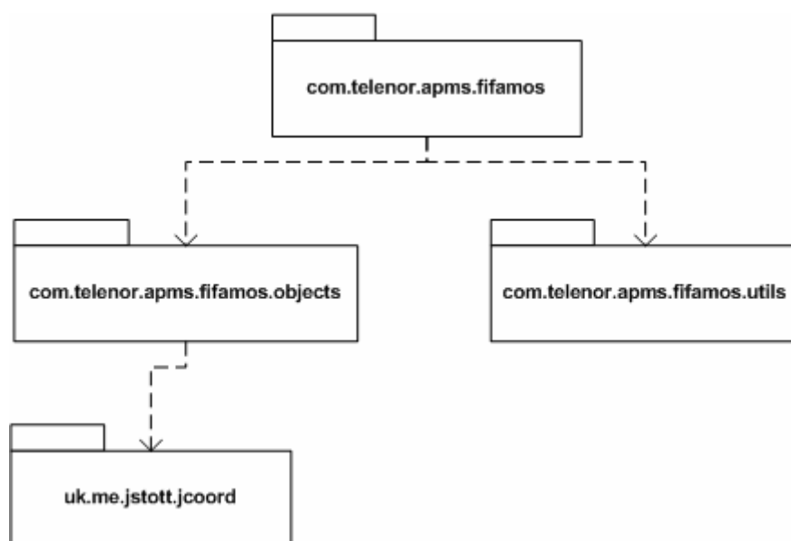
Figure 36: FiFaMoS Context Source package diagram
