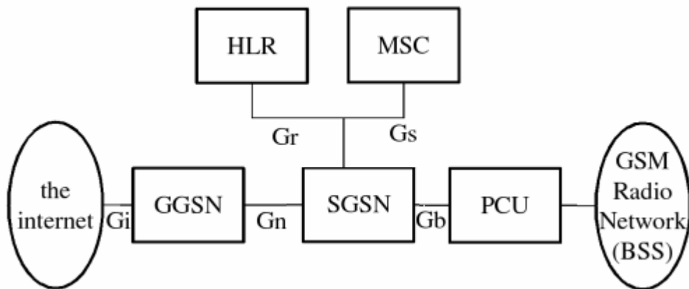
Figure 14: GPRS architecture
