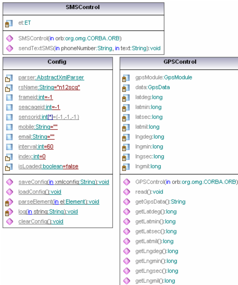
Figure 72: com.telenor.apms.fifamos.n12.utils class diagram
