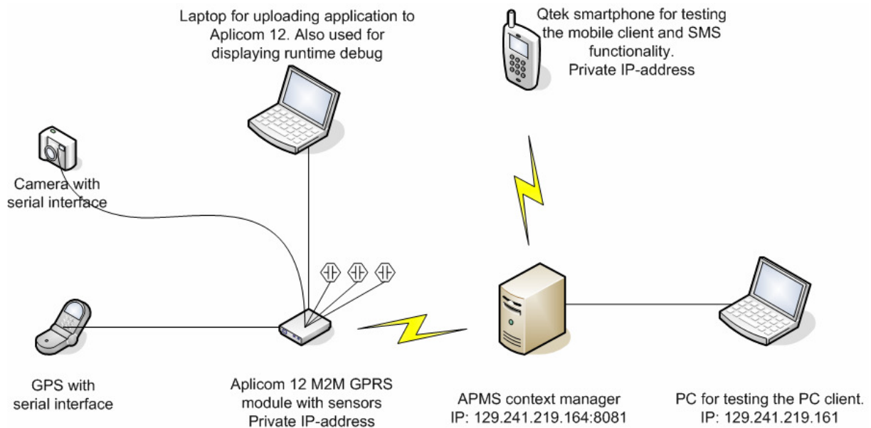
Figure 37: Testing environment
