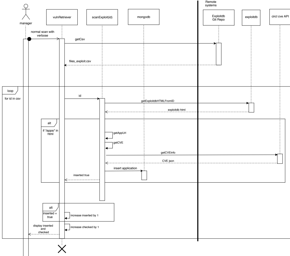
Figure 8: vulnRetriever sequence diagram
