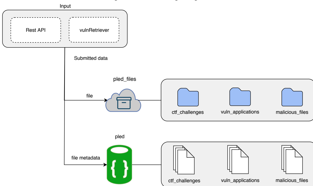
Figure 4: PLED storage diagram
