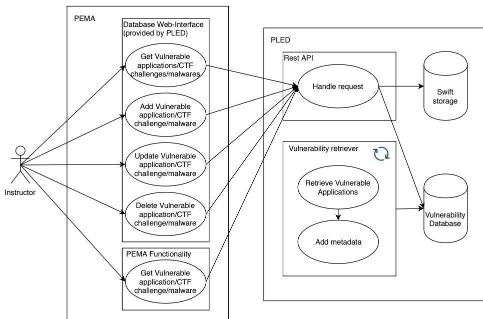
Figure 1: High level use case overview of PLED and PEMA system.
