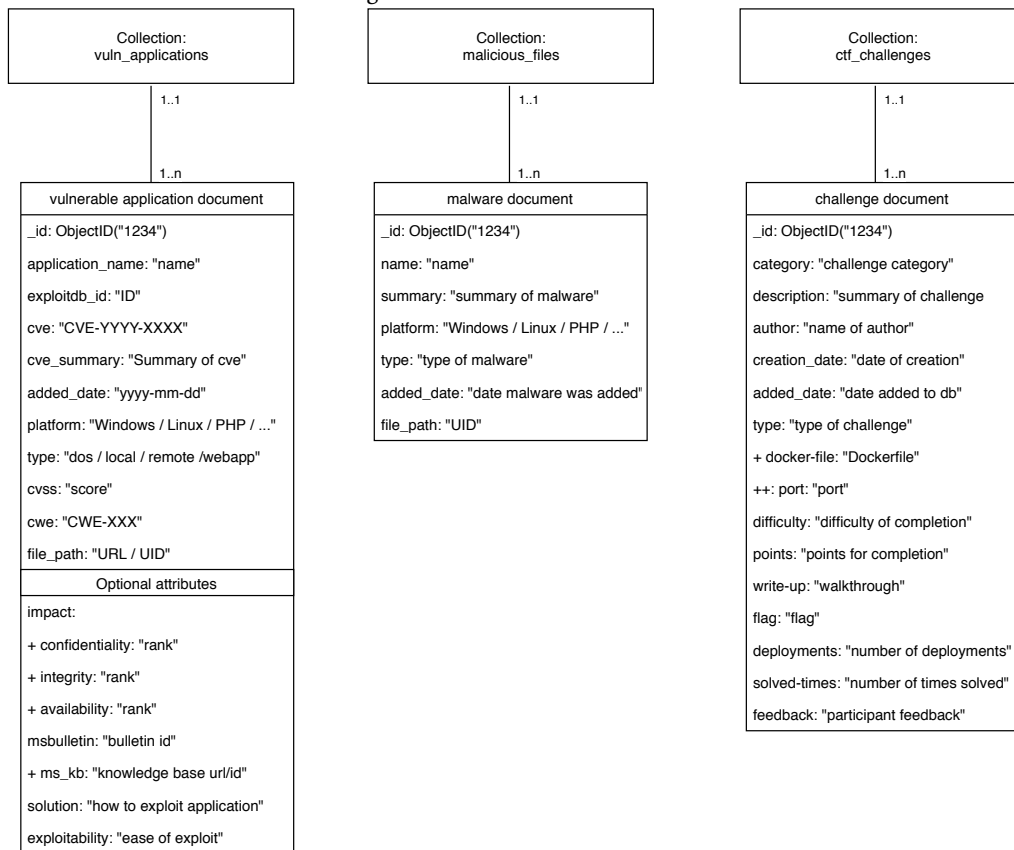
Figure 3: PLED database schema
