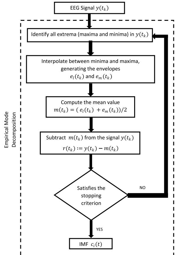
Fig. 1. Flowchart indicating the various stages of the EMD method
