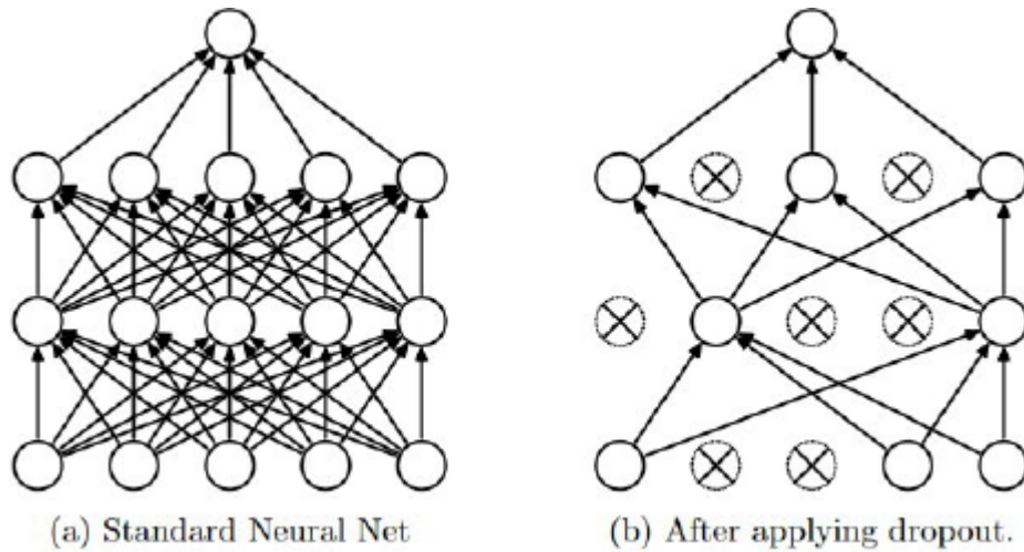
Figure 2.9: Droput schema [14]
