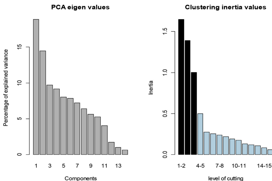
Fig. 6. Contributions of (a) PCA eigenvalues and (b) inertia for hierarchical clustering.
