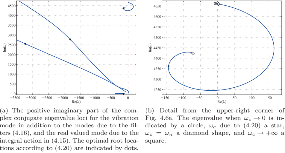
Figure 4.6: Eigenvalue loci for the closed-loop system as a function of the filter cut-off frequency \omega_c . The loci are symmetric about the real axis.
