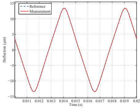
(b) Steady-state measured deflection y_m .
