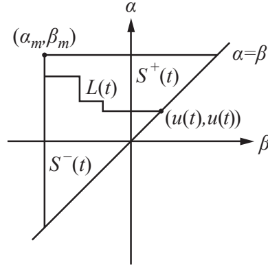
Figure C.3: Preisach plane.
