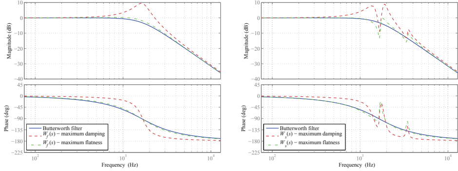
(a) LCR filter, W_f(s) , compared to a Butterworth filter.
