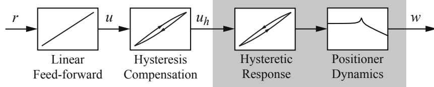
Figure 2.2: Feed-forward tracking control scheme.
