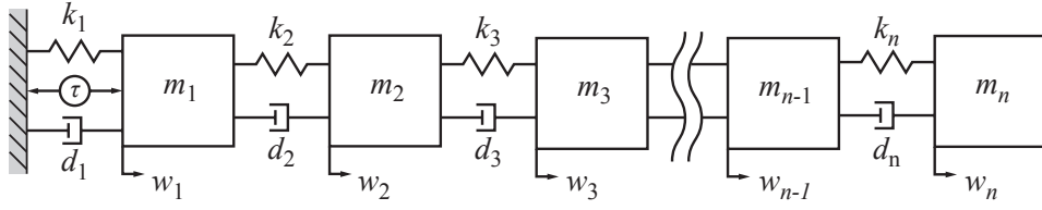
Figure B.5: Clamped-free point masses, with generalized external force.
