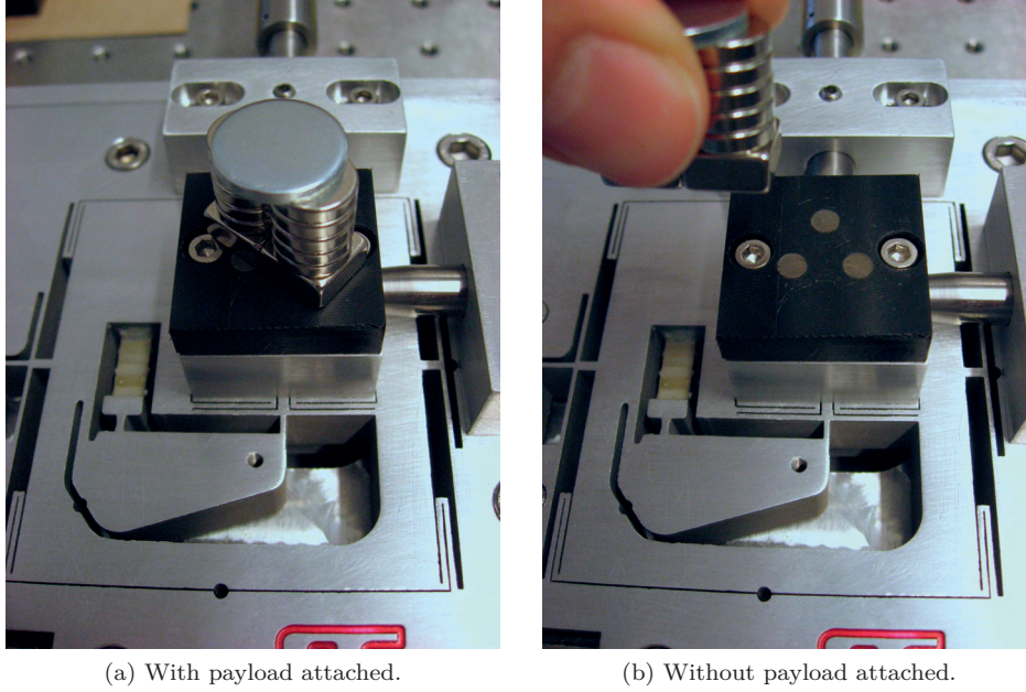
Figure 5.2: Payload configurations.
