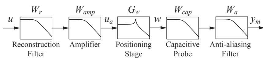
Figure 5.3: Signal chain for the overall system.
