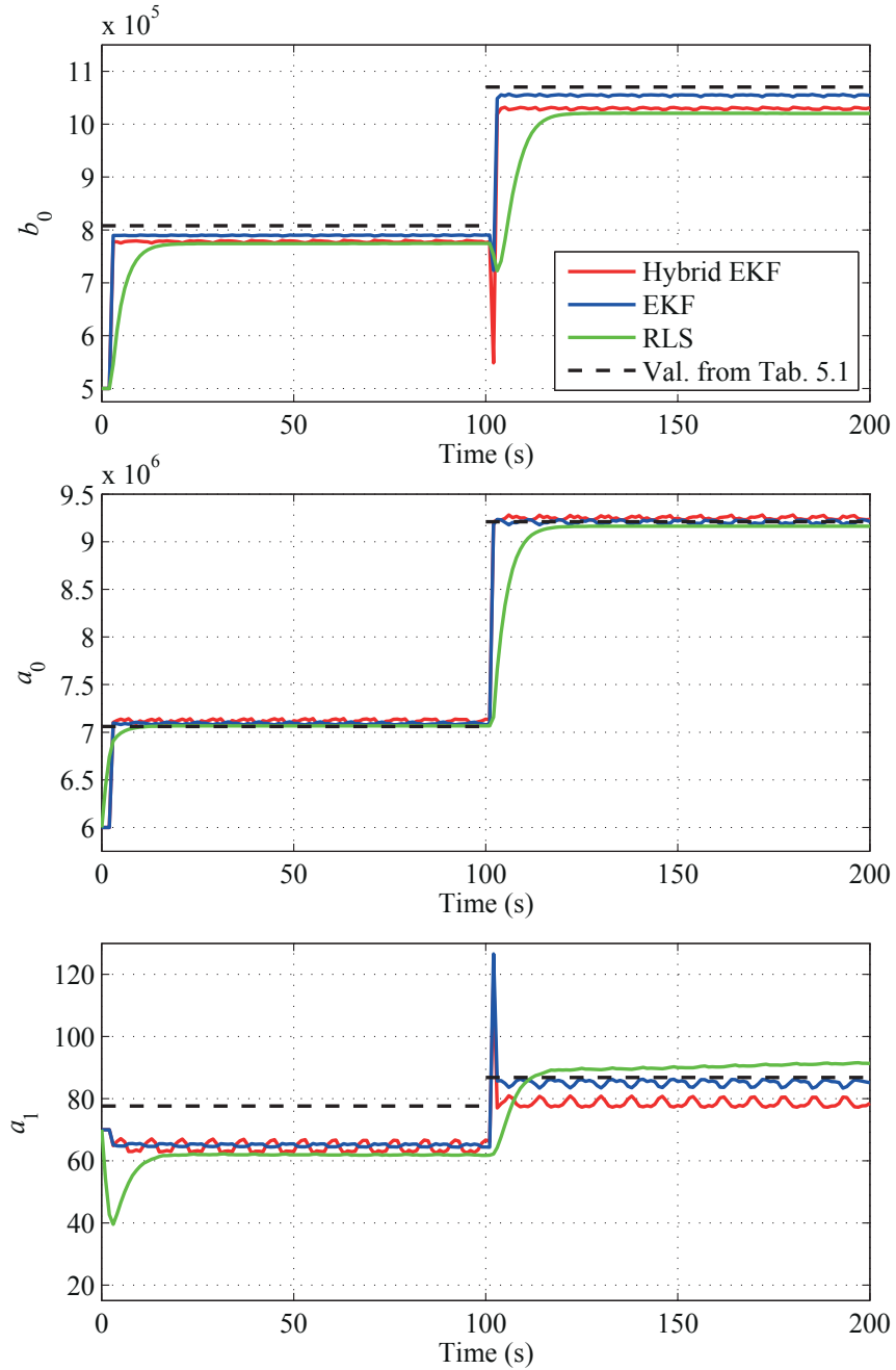
Figure 5.7: Parameter estimates when using PRBS excitation. The time-series have been down-sampled to 1 Hz.
