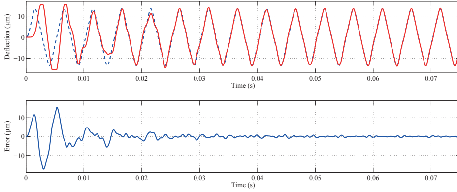
(a) Initial transient measured deflection y_m and measured error \varepsilon .
