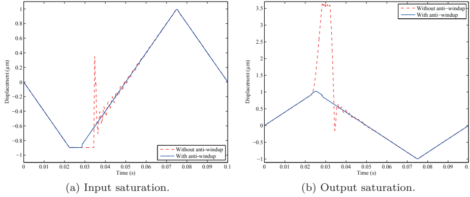
Figure 3.21: Simulated responses to input and output saturation with and without integral anti-windup scheme.
