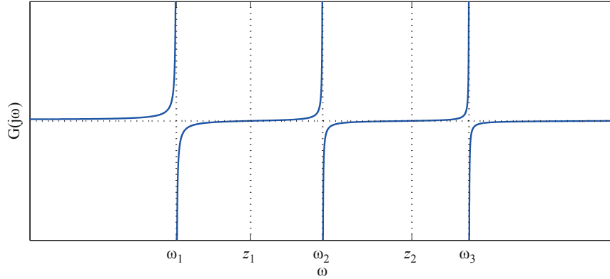
Figure B.3: The real valued Fourier transform G(j\omega) of the transfer-function G(s) .
