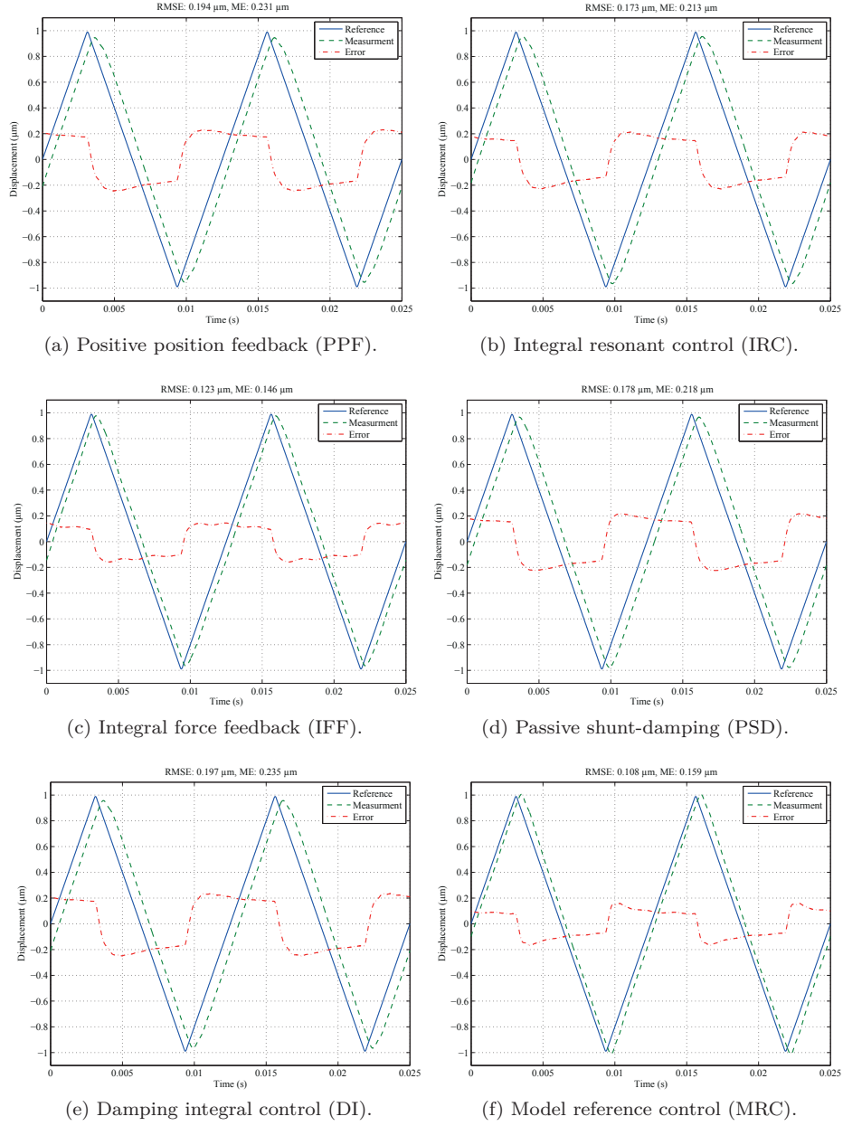
Figure 3.20: Tracking performance.
