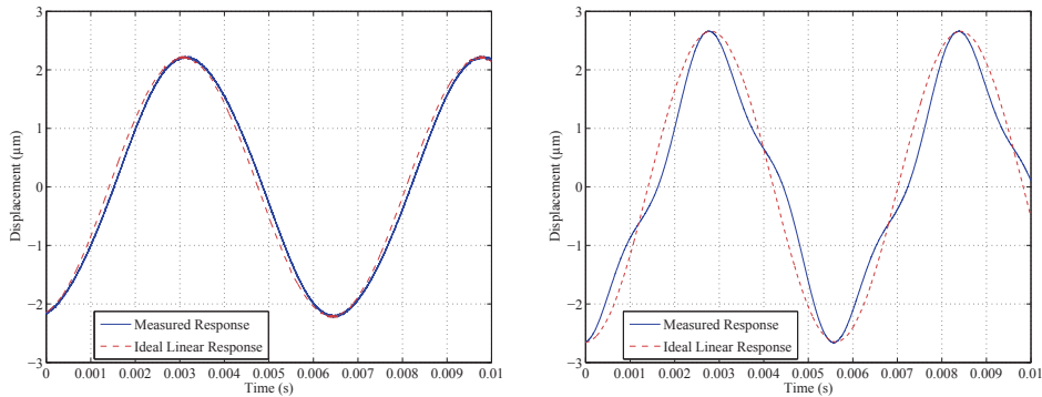
(a) Measured response using a 30 V amplitude sinusoid at 150.0 Hz.
