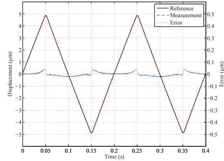
(b) Time-series for the reference signal, and the stationary measured displacement and error when using hysteresis compensation.
