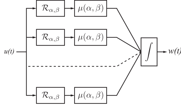
Figure C.2: Preisach model.
