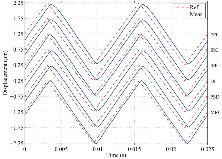
Figure 3.17: Steady-state tracking performance when applying a 1 \mu\text{m} amplitude, 80 Hz triangle-wave reference signal. Displacement measurement signals and reference signals.
