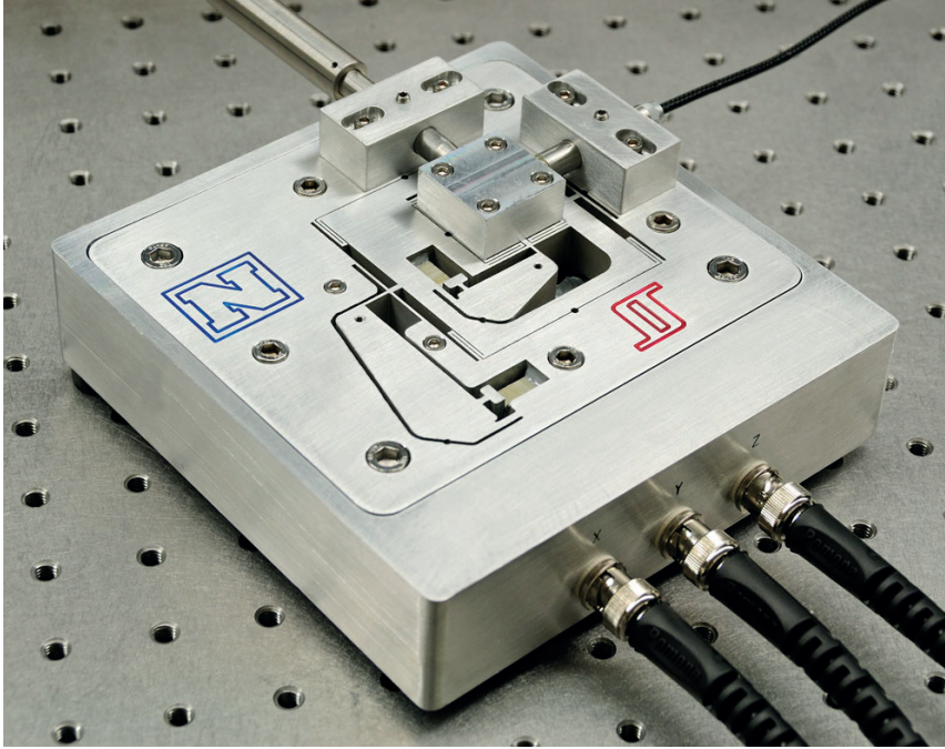
Figure 2.3: Nanositioning stage.
