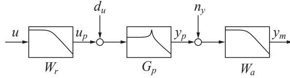
Figure 3.3: System diagram.
