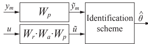
Figure 5.4: Signals fed to identification schemes.
