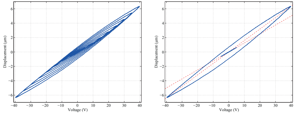
(a) Ensemble of measured hysteresis responses for different voltage signal amplitudes. (b) Change in average linear gain for low amplitude voltage signals and high amplitude voltage signals.
