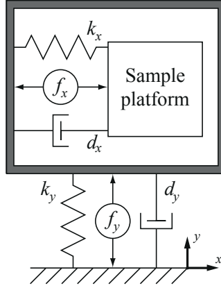
Figure 2.1: Serial kinematic configuration.
