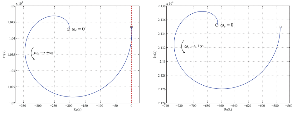
(c) The second vibration mode, cf. Tab. 3.1.
