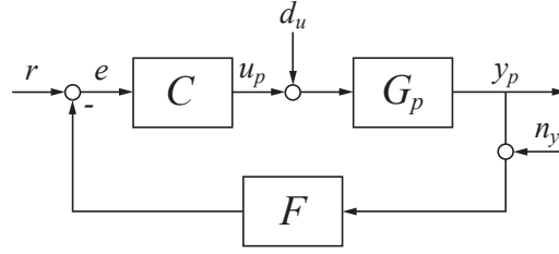
Figure 3.7: General control law structure.
