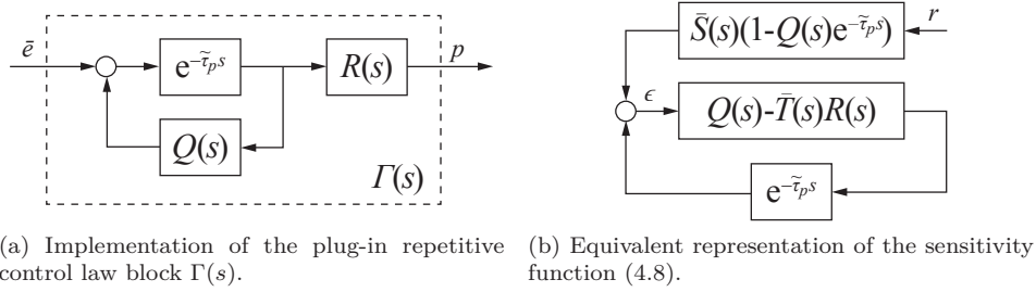
Figure 4.5: Repetitive control scheme block diagrams.
