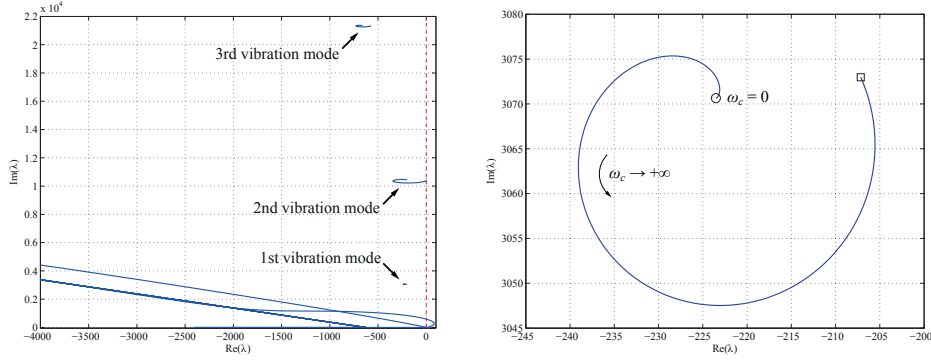
(a) The positive imaginary part of the complex conjugate eigenvalue loci for the vibration modes in addition to the modes due to the filters (3.45), and the real valued mode due to the integral control law (3.44).
