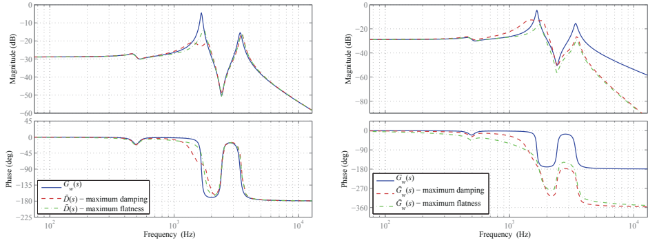
(c) Disturbance attenuation, \bar{D}(s) , compared to the system without the shunt, G_w(s) .
