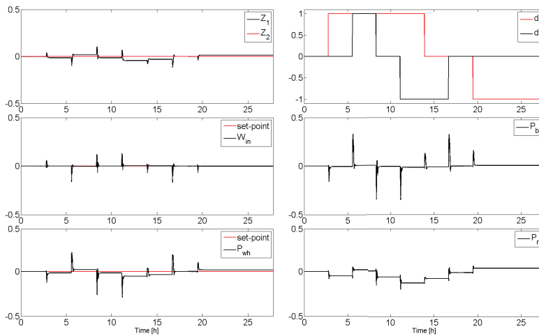
Figure E.6: Control of nonlinear model using P_{wh} and W_{in} as CVs
