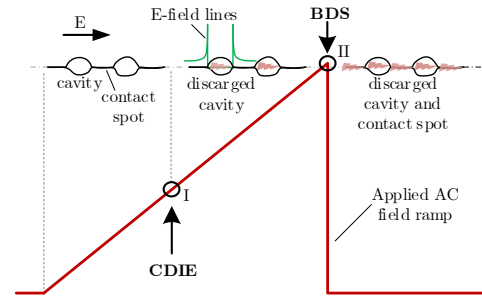
Figure 3. Modeled mechanisms of the cavity discharge and the breakdown of contact spots in parallel with applied field ramp.
