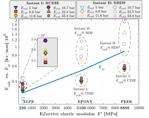
Figure 10. Enhanced field E_{enh} vs. treeing resistance E_{tr} within the covered p_a for each interface: Instant I: Cavity discharge inception. Instant II: Breakdown of contact spots. ( \epsilon_r = 2.3 , G = 20000 \text{ J/m}^2 and r = 0.3 \mu\text{m} for the XLPE; \epsilon_r = 4.6 , G = 20000 \text{ J/m}^2 and r = 0.3 \mu\text{m} for the EPOXY; and \epsilon_r = 2.8 , G = 20000 \text{ J/m}^2 and r = 0.12 \mu\text{m} for the PEEK [2, 6].)
