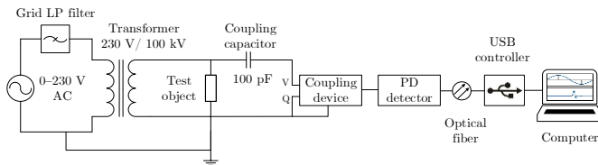
Figure 11. PD test set-up diagram. Coupling device stands for a quadrupole, which is an external measuring impedance for partial discharge measurements.
