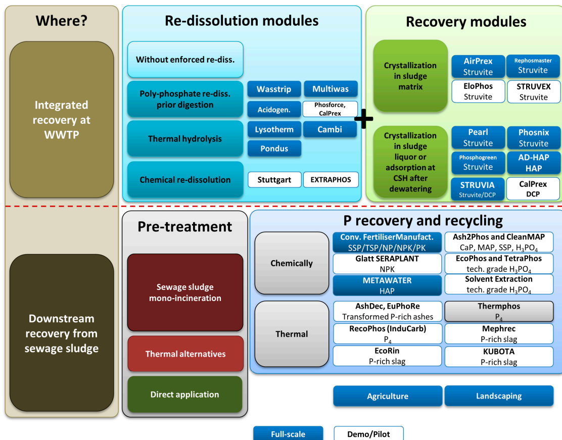
Figure 1. Prominent and already applied concepts for P-recovery and recycling from sewage sludge (Adapted from [21]).
