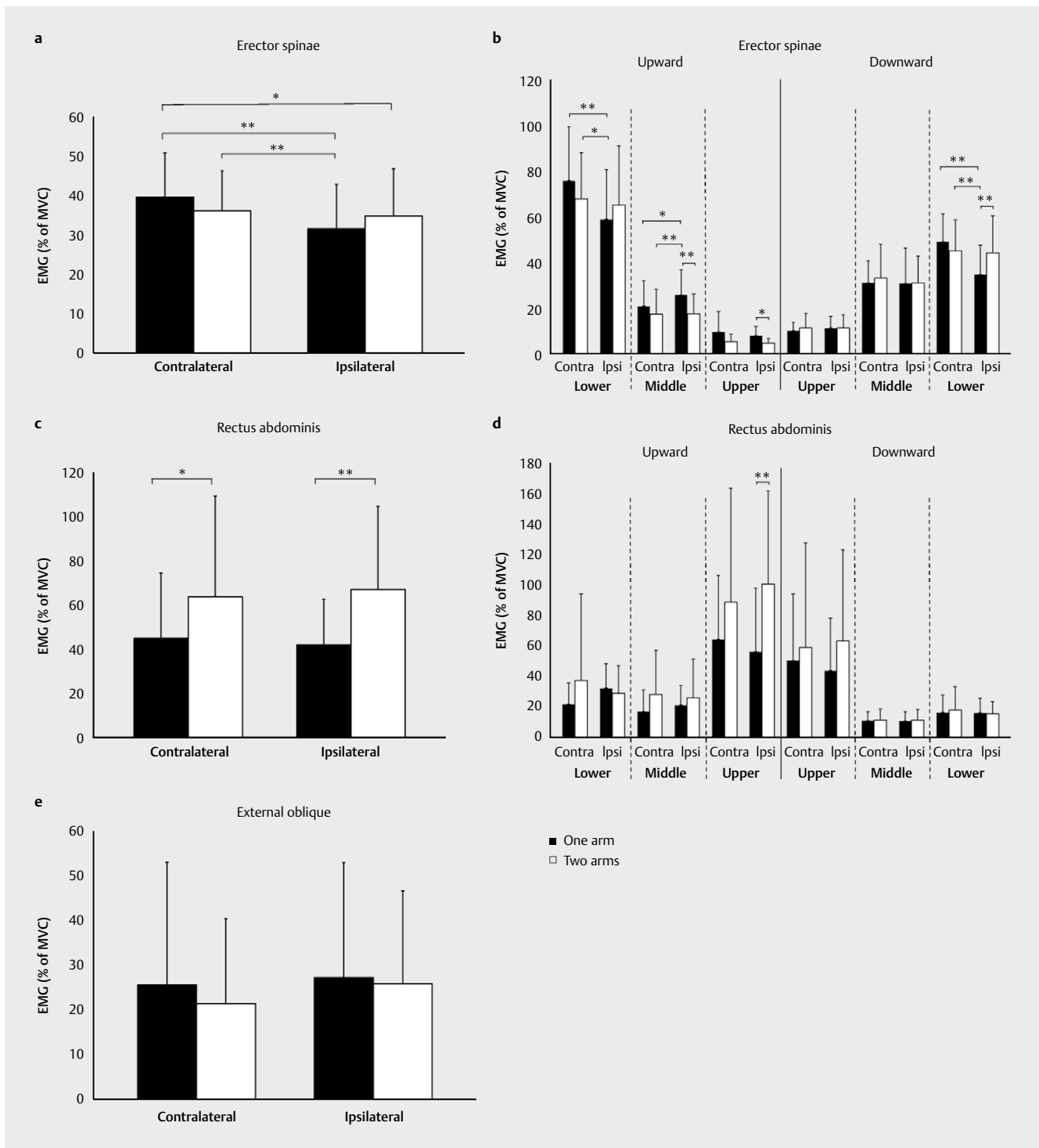
► Fig. 3 Normalized electromyographic (EMG) activation for the whole movement and different phases of the erector spinae muscle (a and b), the rectus abdominis muscle (c and d), and the whole movement of the external oblique muscle e on the contra- and ipsilateral side during the one- and two-armed American kettlebell swing. Values are means ± SD. ** p < 0.01, * p < 0.05.
