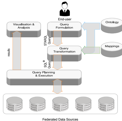
Figure 3. Architecture of our Semantic Platform.
