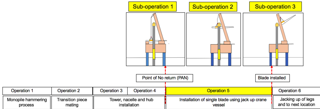
Fig. 1. Different stages of offshore wind turbine installation
