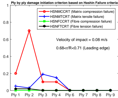
Fig. 12. Ply by Ply Hashin failure criterion (a) 0.08 m/s (No damage initiation)
