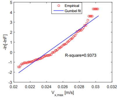
Fig. 8. Data fitting : Gumbel probability paper ( \mu = 0.0241 and \beta = 0.0017 )
