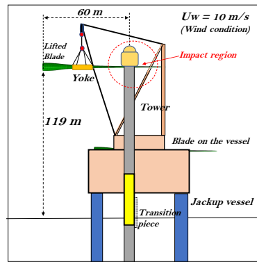
Fig. 7. Case study- Sub-operation 2 of the installation phase
