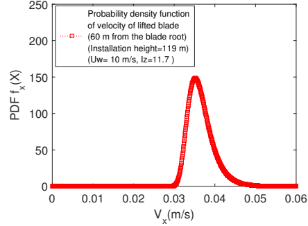
Fig. 9. EVD of impact velocity of the blade
