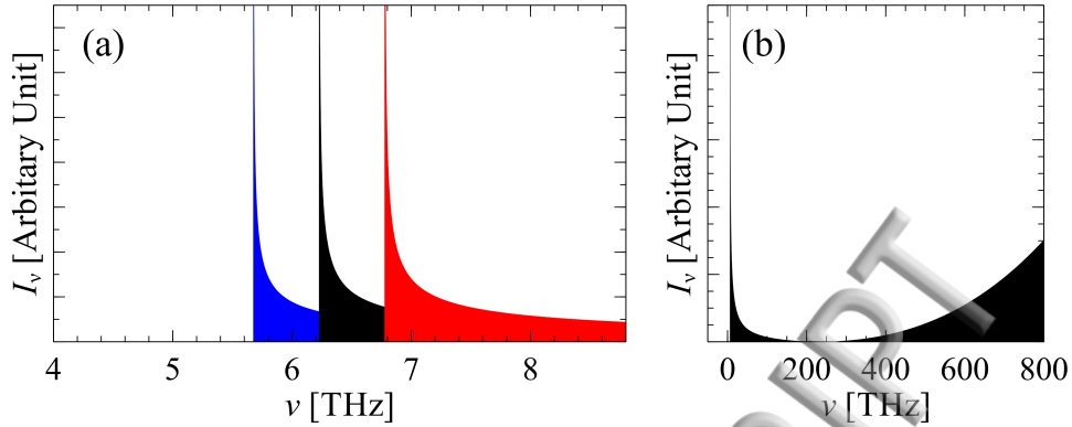
FIG. 4. The calculated photon emission spectra for a (12,-12) CNT in zero magnetic field (black curve) and a magnetic field of B = 5 T, where the red and blue curves correspond to s = 1 and s = -1 respectively, for (a) frequencies of the order of the band gap and (b) for a broad range of frequencies.
