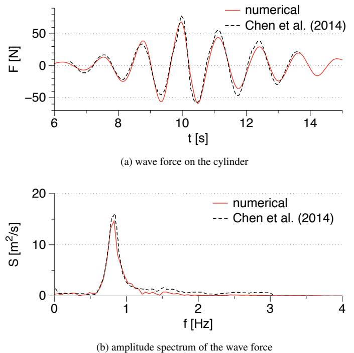
FIGURE 1. Wave forces on a cylinder due to focussed wave of height H = 0.14 m and peak period T_p = 1.22 s
