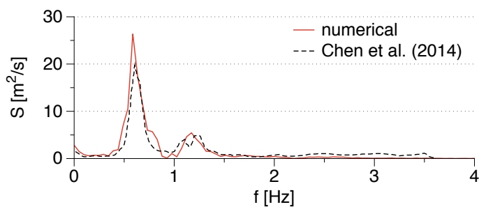
(b) amplitude spectrum of the wave force
