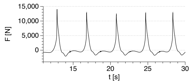
(a) wave force on the cylinder
