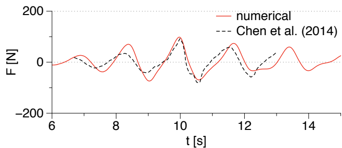
(a) wave force on the cylinder
