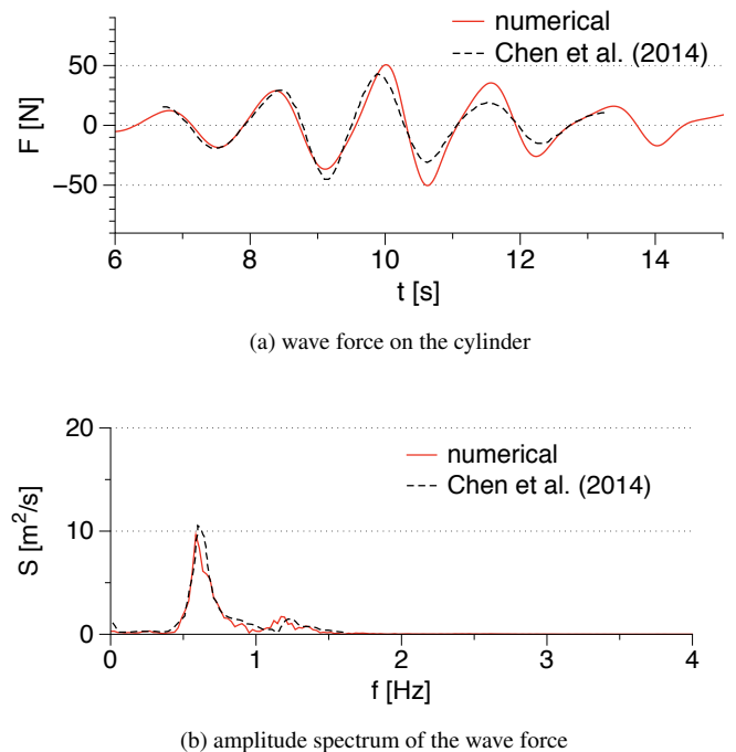
FIGURE 2. Wave forces on a cylinder due to focussed wave of height H = 0.12 m and peak period T_p = 1.63 s
