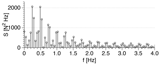
(b) amplitude spectrum of the wave force
