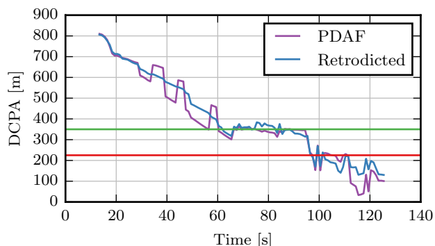
Figure 7. Experiment 1: DCPA for the target vessel. The collision and safety regions are shown in red and green, respectively.
