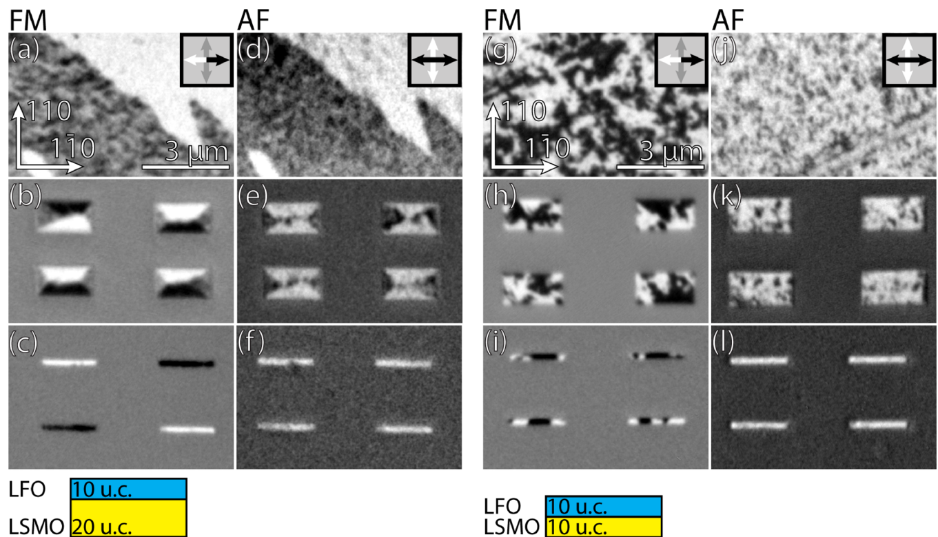
FIG. 2. XMCD- and XMLD-PEEM images showing the FM and AF domain patterns of 10/20 u.c. (a)–(f) and 10/10 u.c. (g)–(l) LFO/LSMO bilayer samples at T < T_C ( T = 100 K). Images in (a), (d), (g), and (j) show the domain pattern for blanket films; (b), (e), (h), and (k) the domain patterns for 1 \times 2 \mu\text{m}^2 rectangles; and (c), (f), (i), and (l) the domain patterns for 200 \text{ nm} \times 2 \mu\text{m} line segments. Legends showing the correspondence between X-PEEM domain contrast and direction of magnetization apply for all three images in each column.
