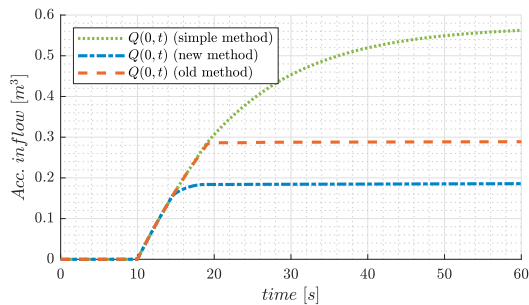
Fig. 6. Accumulated net inflow.
