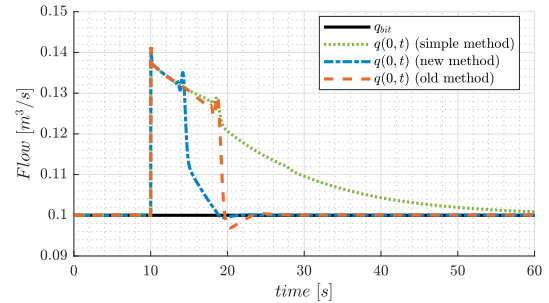
Fig. 3. Bottom-hole flow.
