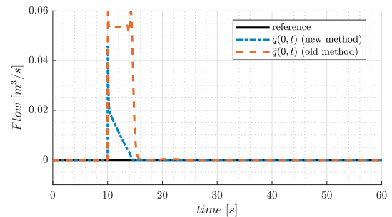
Fig. 5. Bottom-hole flow estimation error.
