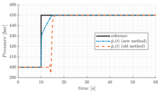
Fig. 7. Reservoir pressure estimate.
