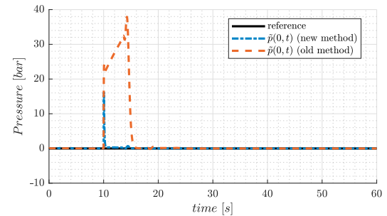
Fig. 4. Bottom-hole pressure estimation error.
