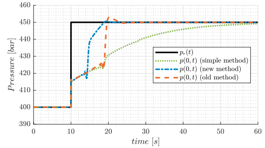
Fig. 2. Bottom-hole pressure.
