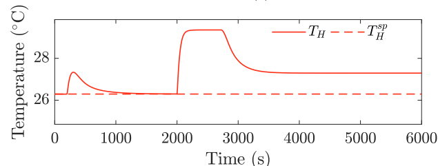
(c) Two controllers with different setpoints.
