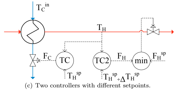
Fig. 7. Analyzed control structures for cooler.
