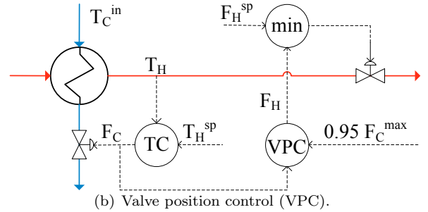
(b) Valve position control (VPC).
