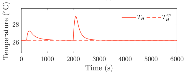
(a) Split Range Control (SRC).
