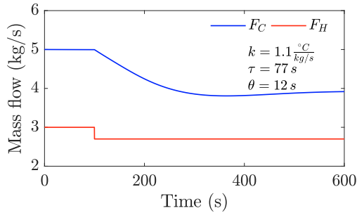
Fig. 6. Response in F_C for a step in F_H ; used to tune the valve position controller (VPC).
