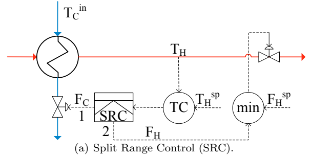
(a) Split Range Control (SRC).
