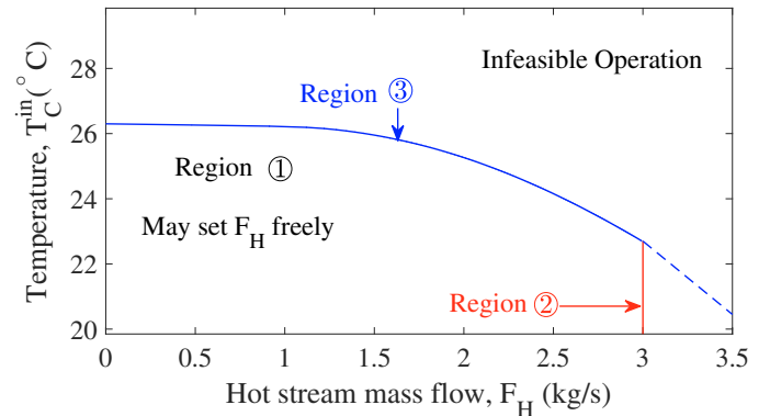
Fig. 4. Active constraint regions for the cooler.
