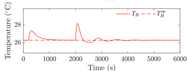
(b) Valve position control (VPC).
