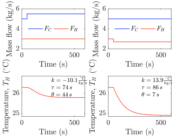
Fig. 5. Open-loop response in T_H for a step in F_C and F_H .
