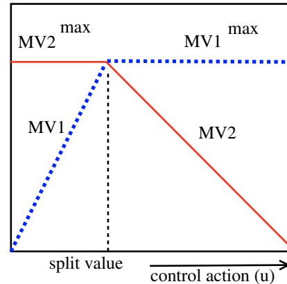
Fig. 2. Simple representation of split range control (SRC).
