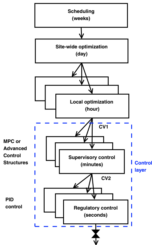
Fig. 1. Typical control hierarchy in a process plant (Skogestad, 2004)
