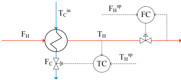
Fig. 3. Cooler with temperature and flow control 1 .
