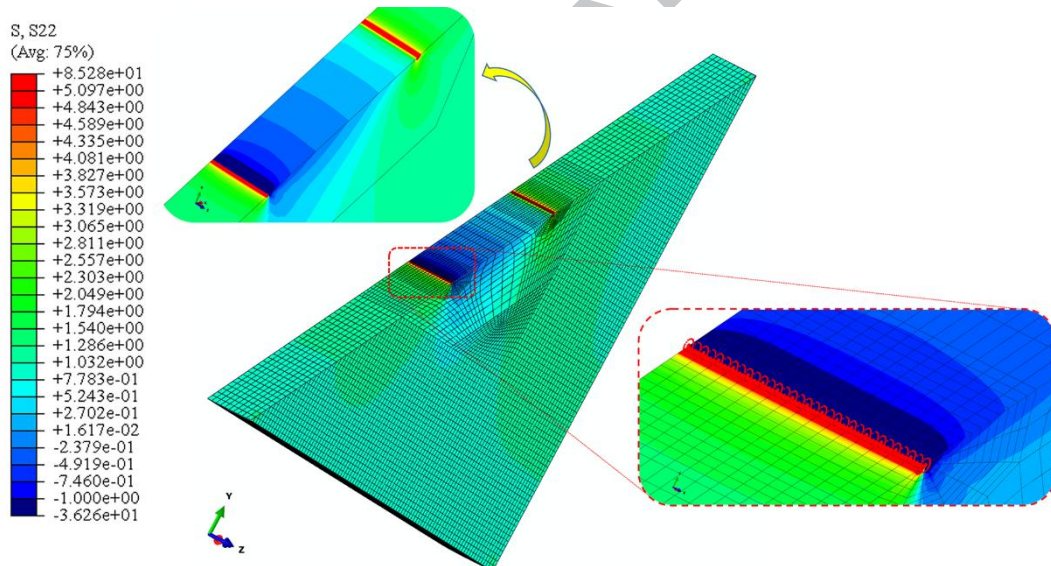
Figure 13. Contour plots of the principal stress, \sigma_{22} , for the undeformed and deformed configurations, respectively, with highlight of the stress scenario for a single cracked zone.
