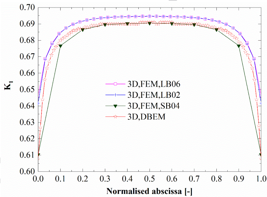
Figure 17. 3D Beasy and Zencrack normalised K_I comparison.
