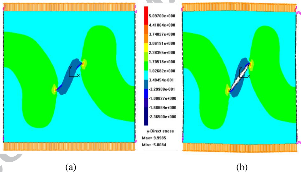
Figure 8. Principal stresses \sigma_{22} on the undeformed plot (a) and on the deformed plot (b).
