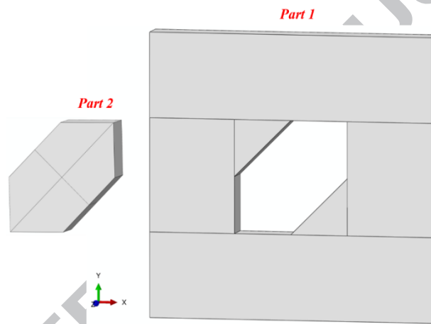
Figure 6. Highlighting of the Part 1 and Part 2 of the assembly. Tie constraint conditions have been applied at interfaces between the two parts.
