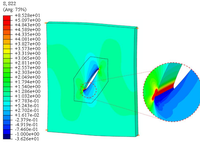
Figure 13. Contour plots of the principal stress, \sigma_{22} , for the undeformed and deformed configurations, respectively, with highlight of the stress scenario for a single cracked zone.
