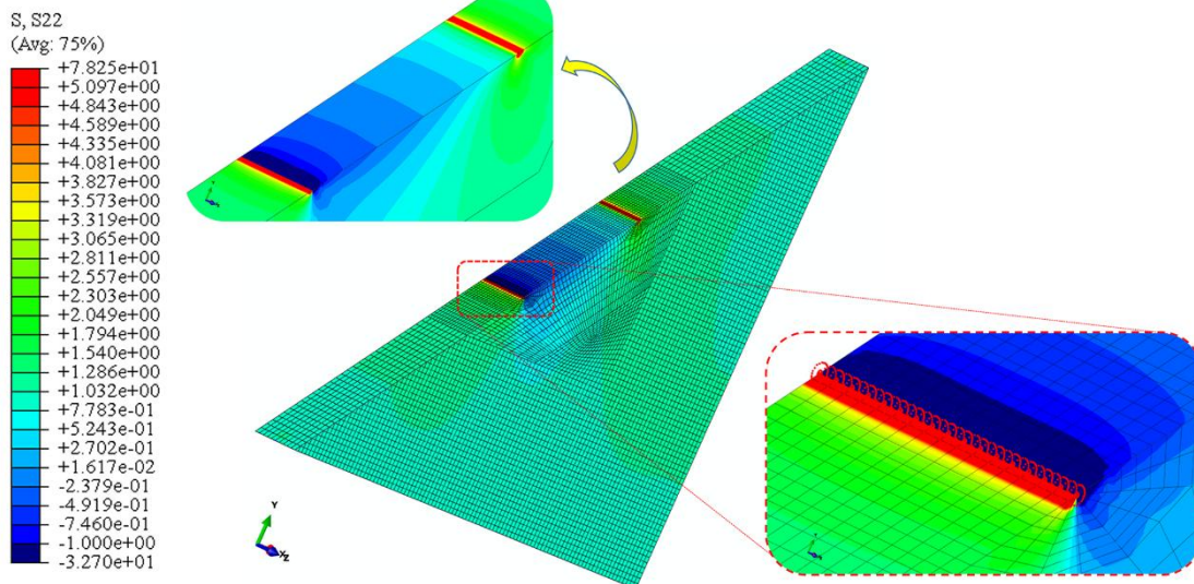
Figure 16. Contour plot of principal stress, \sigma_{22} , for the 45° cut square plate with highlight of J-paths along the crack front.
