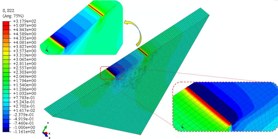
Figure 12. Contour plot of the principal stress, \sigma_{22} , for the 45° cut square plate with highlight of the J-paths along a crack front.
