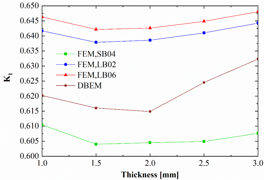
Figure 19. Comparison of the normalized K_I at free surface and with increasing thickness.
