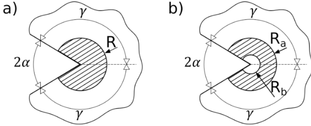
Figure 4. Control volumes in the approach based on the deviatoric SED (a) and in the modified version of the approach based on the deviatoric SED (b) [27].
