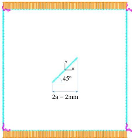
Figure 7. Highlight of the mesh adopted for the square plate with the 45^\circ tilted crack with boundary conditions.
