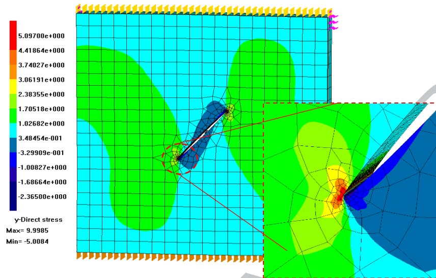
Figure 9. Contour plot of principal stresses, \sigma_{yy} , on deformed plot with highlight of the crack front.
