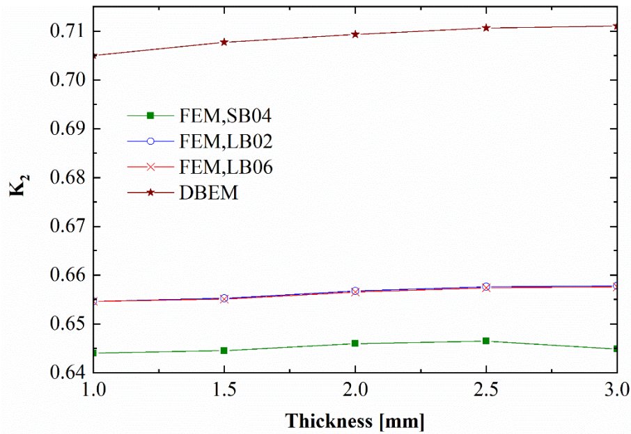
Figure 22. Comparison of the K_2 calculated at midside position of the crack front and with increasing thickness.
