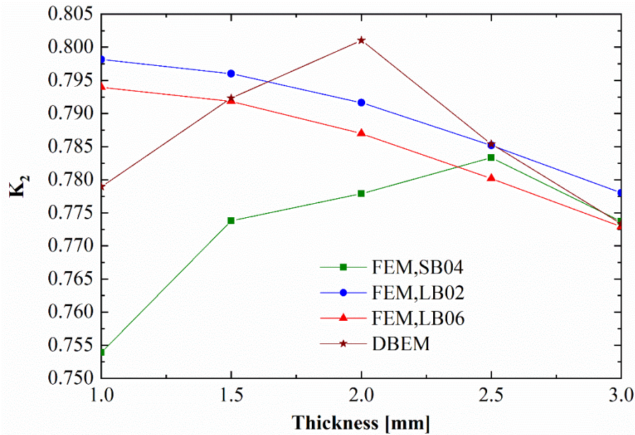
Figure 20. Comparison between the K_2 values, obtained from the FEM-DBEM based analyses, calculated at the free surfaces and with increasing thickness.
