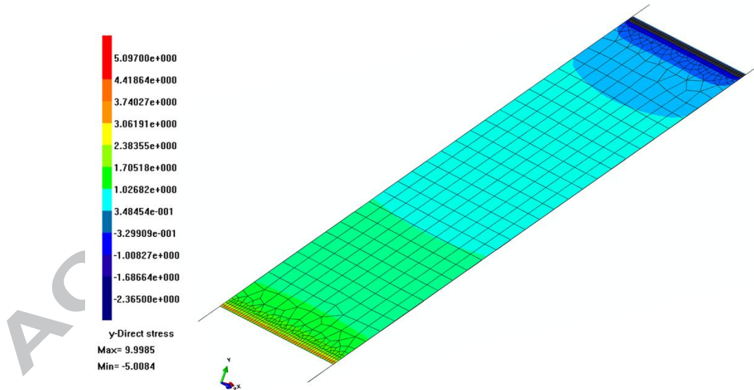
Figure 10. Contour plot of \sigma_{yy} with highlight of a crack front.
