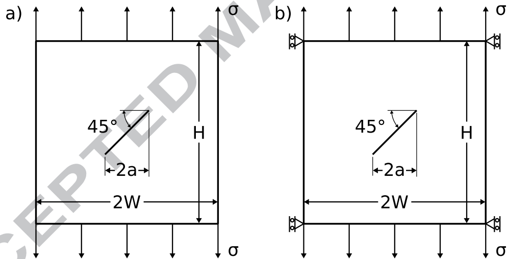
Figure 1. Loaded square plate with the 45° tilted crack (a) and loads and boundary conditions applied in FEA (b).
