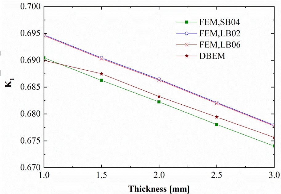
Figure 21. Comparison of the K_1 values calculated at midside position of the crack front and with increasing thickness.
