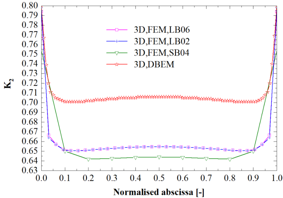
Figure 18. 3D Beasy and Zencrack normalized K_2 comparison.
