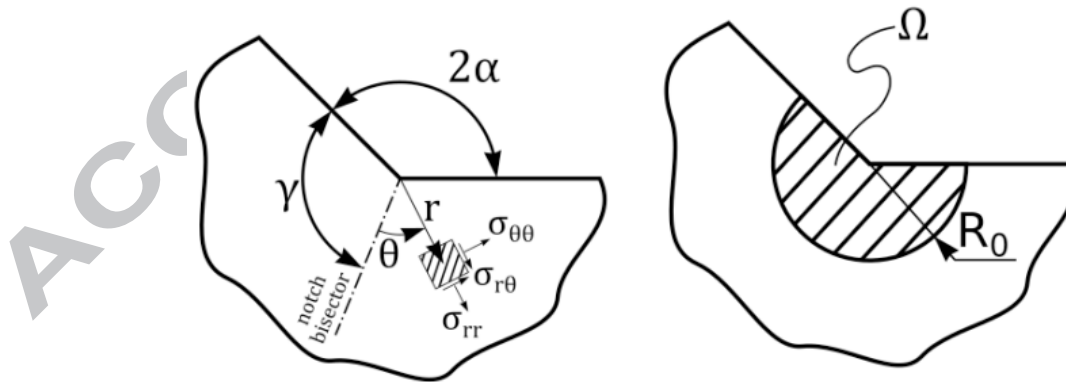
Figure 2. Polar coordinate system centered at the notch tip [27].
