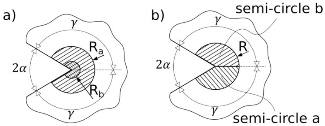
Figure 3. Control volumes in the Lazzarin et al. approach (a) and in the Treifi and Oyadiji approach (b) [27].
