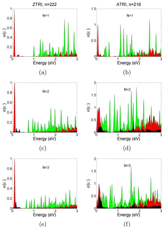
FIG. 5: Optical absorption cross section for multilayer ZTRI and ATRI PQDs. Three colours (online only) represent the three absorption cross sections, green for \sigma_x , red for \sigma_y , and black for \sigma_z .
