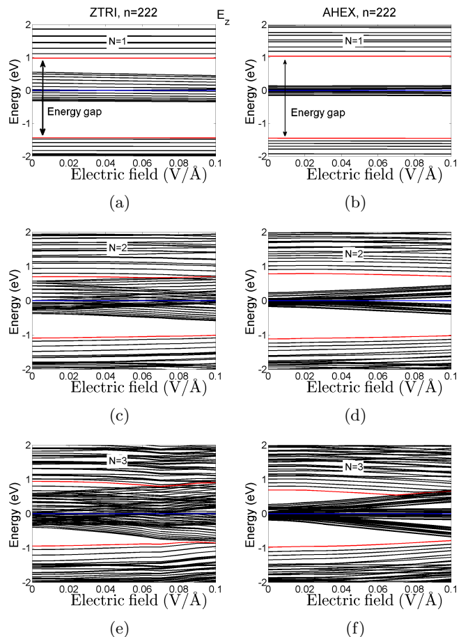
FIG. 2: Electronic energy levels as a function of perpendicular electric field for ZTRI (a, c, e) and for AHEx (b, d, f) with the total number of layers N = 1, 2, and 3 .
