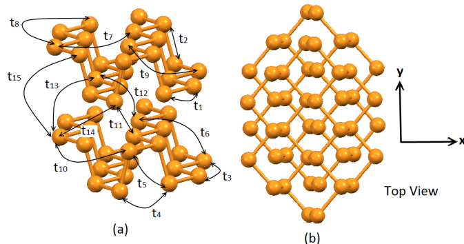
FIG. 1: (a) The geometrical structure and tight-binding hopping parameters t_{ij} of phosphorene bilayer. (b) Top view of the bilayer PQD with n_l = 48 atoms.
