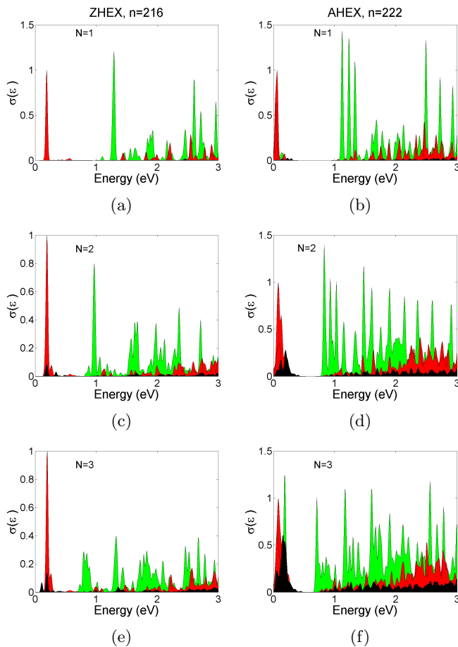
FIG. 13: The optical absorption cross section for (a, c, e) ZHEX and (b, d, f) AHEX N -layer PQDs.
