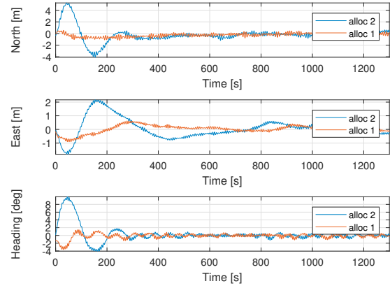
Fig. 3. The position and heading of the vessel recorded during the test case run for both allocator 1 and 2.
