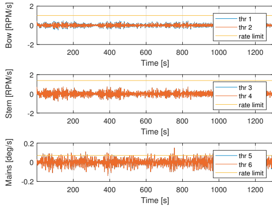
Fig. 5. Shows the change rate of the commands issued to each thruster.
