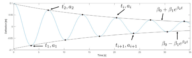
Fig. 4. Identification of decay-rate from decay tests.
