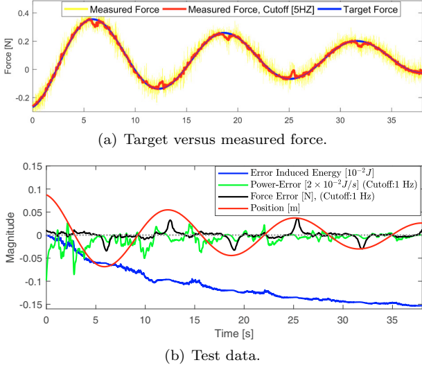
Fig. 5. Trajectory and errors for decay-test in x-direction. ( k_x=4\text{N/m} )
