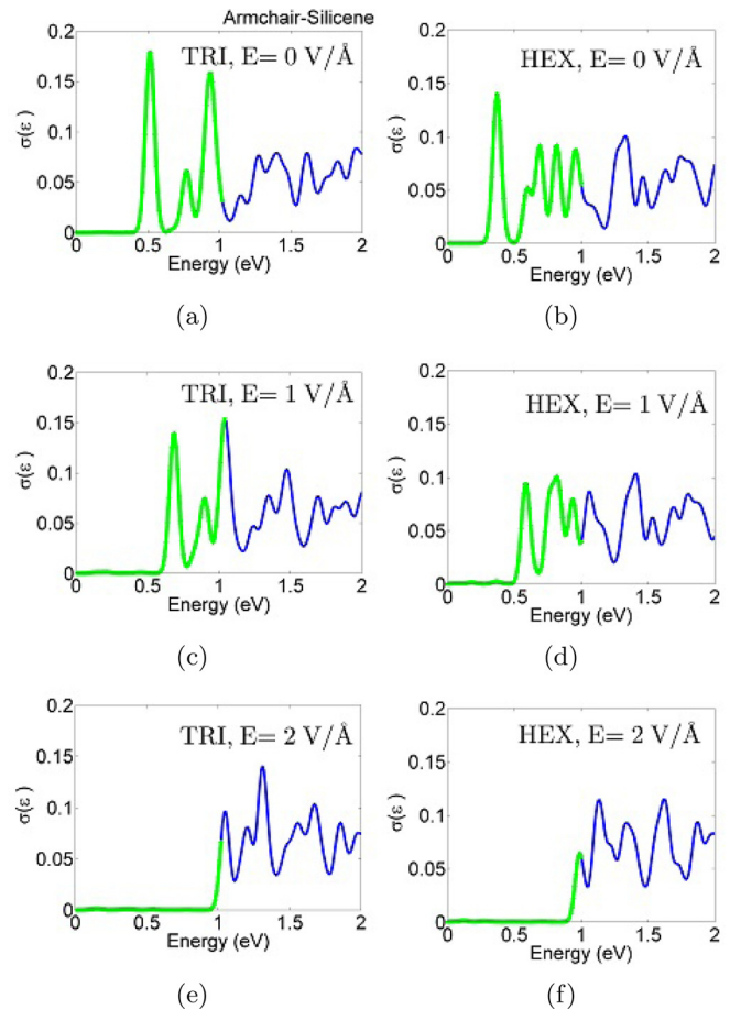
FIG. 6. Optical absorption spectra for armchair silicene QDs of triangular (a), (c), (e) and hexagonal (b), (d), (f) shapes, consisting of 468 and 762 atoms and having edge length L \approx 80 \text{ \AA} and L \approx 42 \text{ \AA} , respectively.
