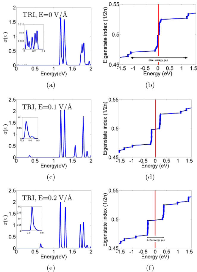
FIG. 7. Optical absorption spectra (a), (c), (e) and energy levels (b), (d), (f) of a triangular bilayer graphene QD made of 222 atoms per layer ( L \approx 34 \text{ \AA} ) at different electric fields. The insets show zoomed in absorption peaks below 0.8 \text{ eV} .
