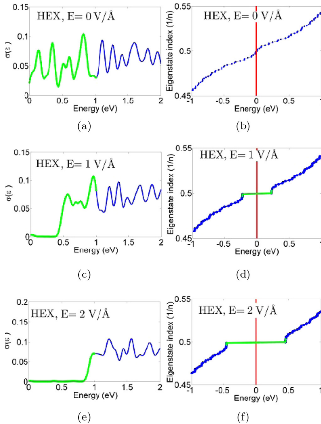
FIG. 5. The same as Fig. 4, but for a hexagonal (HEX) silicene QD containing 864 atoms ( L \approx 45 \text{ \AA} ) at different electric fields.
