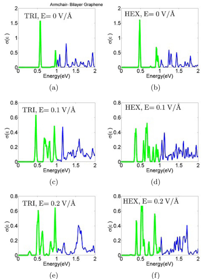
FIG. 10. Optical absorption spectra for armchair bilayer graphene QDs of triangular (a), (c), (e) and hexagonal (b), (d), (f) shapes with 720 ( L \approx 64 \text{ \AA} ) and 762 ( L \approx 27 \text{ \AA} ) atoms per layer, respectively.
