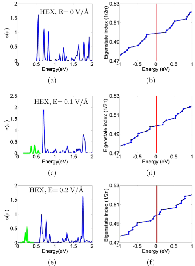
FIG. 8. The same as Fig. 7, but for a hexagonal bilayer graphene QD containing 216 atoms per layer ( L \approx 14 \text{ \AA} ) at different electric fields.
