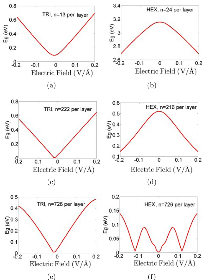
FIG. 9. Energy gap dependence on the applied electric field in triangular (a) L \approx 7.4 \text{ \AA} , (c) L \approx 34 \text{ \AA} , (e) L \approx 64 \text{ \AA} and hexagonal (b) L \approx 4.1 \text{ \AA} , (d) L \approx 14 \text{ \AA} , (f) L \approx 26 \text{ \AA} bilayer graphene QDs.
