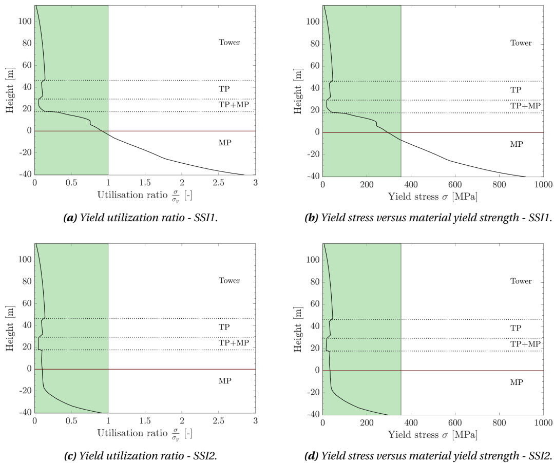
Figure 5.36: Global yield limit check for the nonlinear elastic soil-structure interaction model (SSII, 5.36a and 5.36b) and the nonlinear inelastic series hysteretic-viscous damping model (SSI2, 5.36c and 5.36d) under wind, wave and earthquake loads, when the turbine is in normal operation mode.
