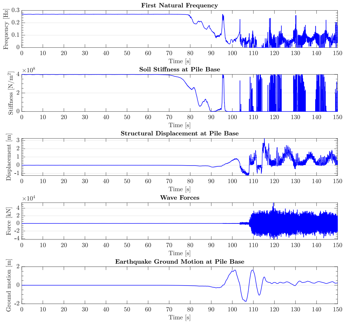
Figure 5.71: Change in first natural frequency over time, in comparison to the change in soil stiffness, change in pile base deflection and wave forcing, for the nonlinear elastic soil-structure interaction model to wind, waves and the Abnormal Level Earthquake, after the turbine performed an emergency break.
