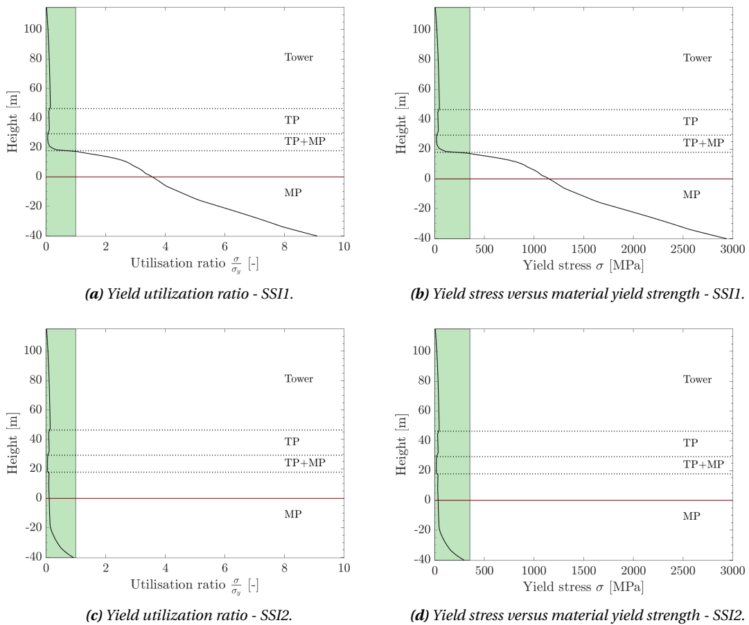
Figure 5.76: Global yield limit check for the nonlinear elastic soil-structure interaction model (SSII, 5.76a and 5.76b) and the nonlinear inelastic series hysteretic-viscous damping model (SSI2, 5.76c and 5.76d) under wind, wave and Abnormal Level Earthquake loads, when the turbine is in normal operation mode.
