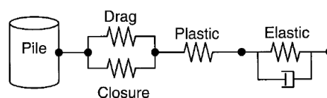
Figure 2.7: The nonlinear elastoplastic p - y element of the series hysteretic-viscous damping model by Boulanger et al. [13].
