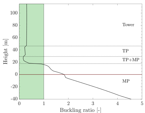
(a) Buckling ratio versus limit - SSI1.
