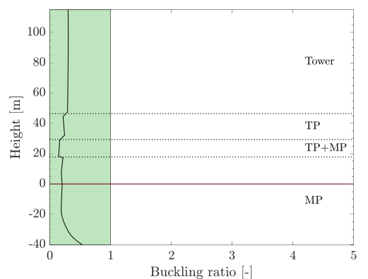
(b) Buckling ratio versus limit - SSI2.
