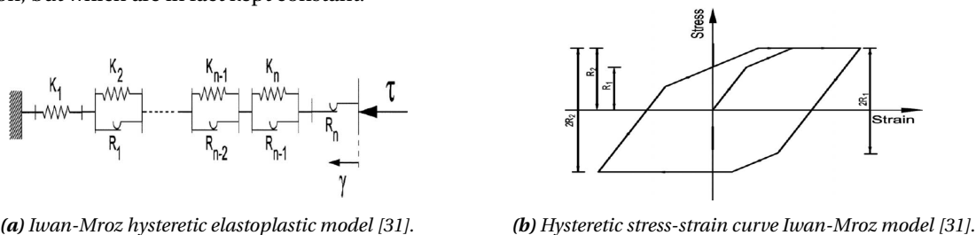
Figure 4.16: Nonlinear soil stress-strain Iwan-Mroz model used in NERA nonlinear site response analysis.
