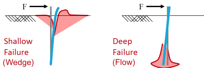
Figure 3.3: Shallow failure versus deep failure in sand [43].
