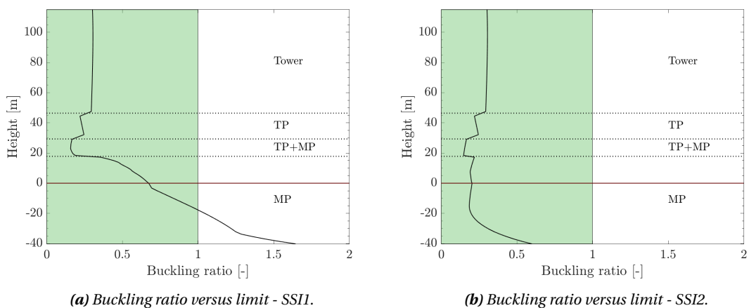
Figure 5.39: Global buckling limit check for the nonlinear elastic soil-structure interaction model (SSII, 5.39a) and the nonlinear inelastic series hysteretic-viscous damping model (SSI2, 5.39b) under wind, wave and earthquake loads, when the turbine is in emergency shutdown mode.
