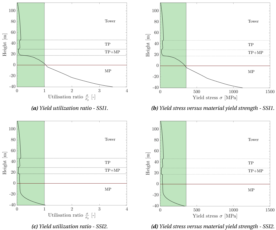
Figure 5.38: Global yield limit check for the nonlinear elastic soil-structure interaction model (SSII, 5.38a and 5.38b) and the nonlinear inelastic series hysteretic-viscous damping model (SSI2, 5.38c and 5.38d) under wind, wave and earthquake loads, when the turbine is in emergency shutdown mode.
