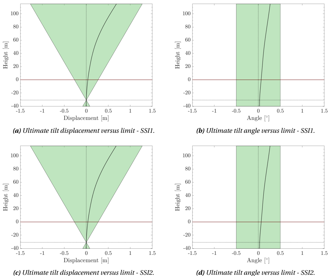
Figure 5.14: Tilt limit check for the nonlinear elastic soil-structure interaction model (SSI1, 5.14a and 5.14b) and the nonlinear inelastic series hysteretic-viscous damping model (SSI2, 5.14c and 5.14d) under wind and wave loads only, when the turbine is in normal operation mode.
