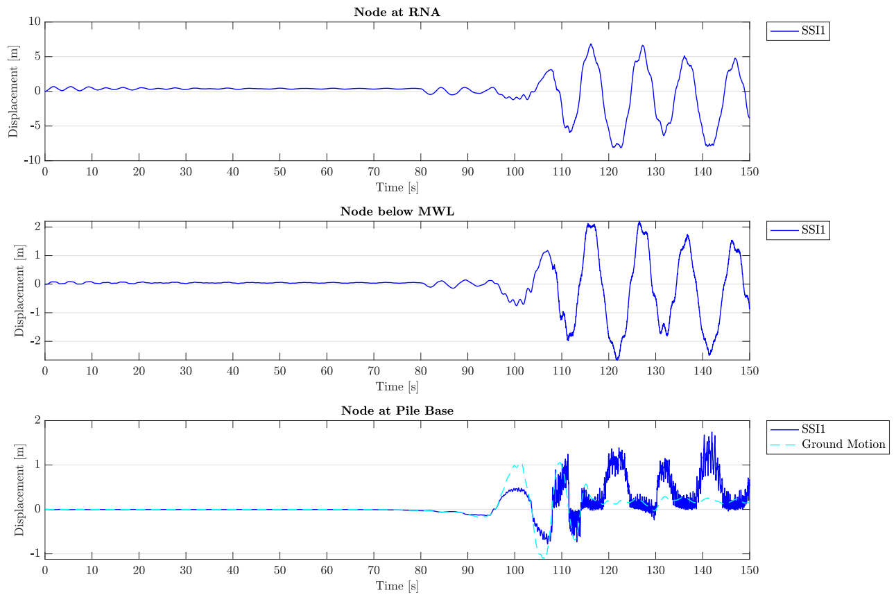
Figure 5.44: Lateral pile displacement time history for the nonlinear elastic soil-structure interaction model (SSII), for co-directional loading by wind, waves and the Extreme Level Earthquake, under shutdown conditions (DLC 3-S). Time history depicted for the RNA node, the node directly below maximum water level, and the node at the pile base below mudline. As a reference, the ground motion is shown versus the pile displacement below mudline.
