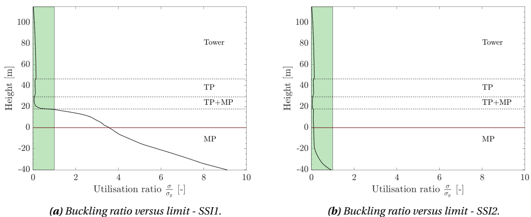
Figure 5.77: Global buckling limit check for the nonlinear elastic soil-structure interaction model (SSII, 5.77a) and the nonlinear inelastic series hysteretic-viscous damping model (SSI2, 5.77b) under wind, wave and Abnormal Level Earthquake loads, when the turbine is in normal operation mode.
