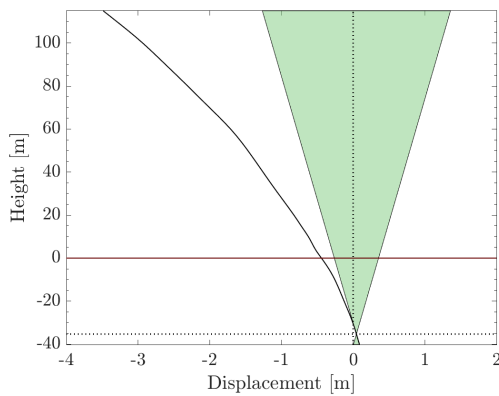
(a) Ultimate tilt displacement versus limit - SSI1.
