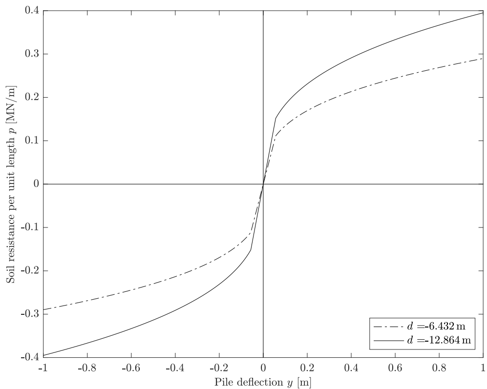
Figure 3.11: P - y behaviour in the clay layer, at the start and at the end of the layer.
