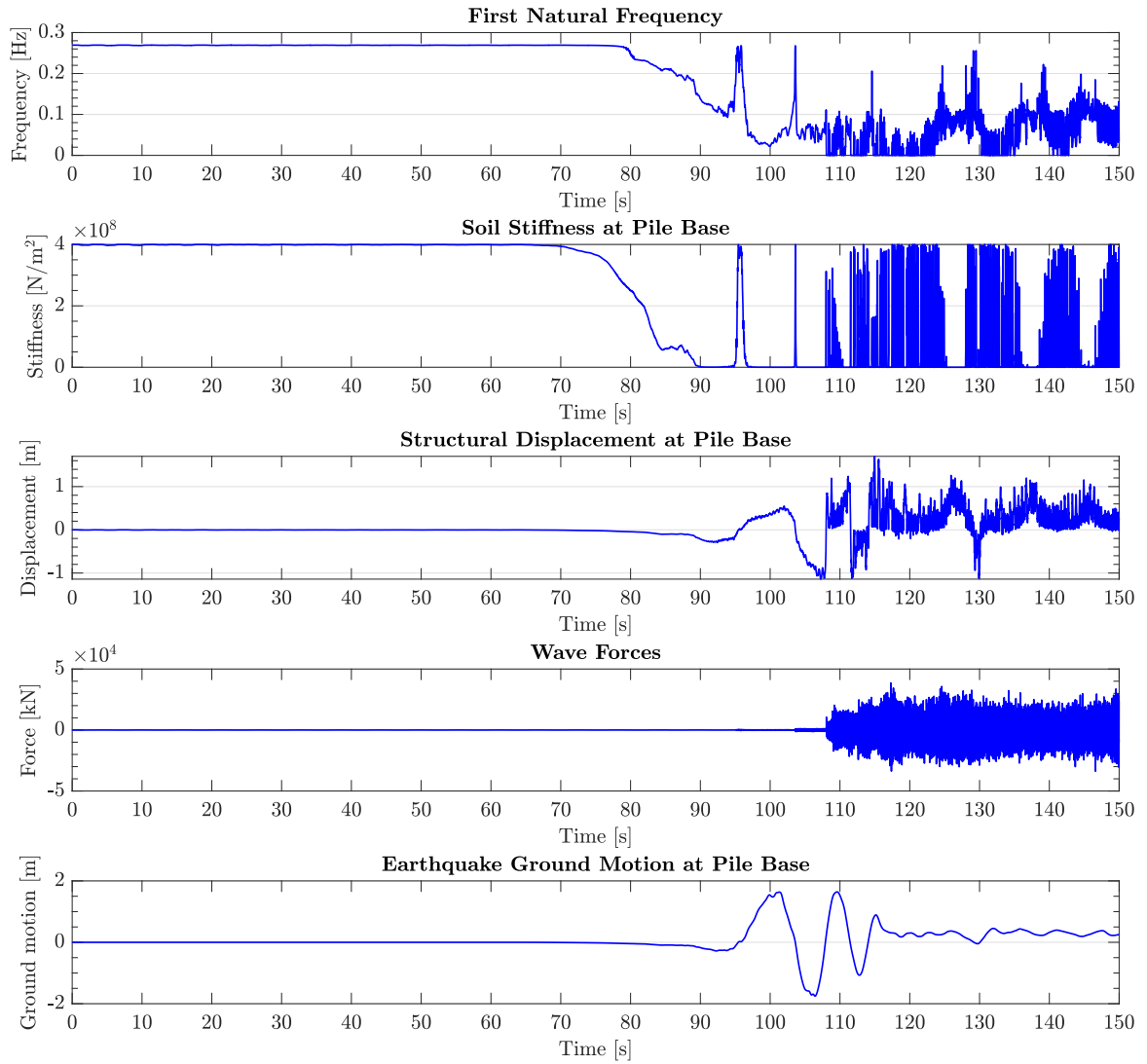
Figure 5.67: Change in first natural frequency over time, in comparison to the change in soil stiffness, change in pile base deflection and wave forcing, for the nonlinear elastic soil-structure interaction model to wind, waves and the Abnormal Level Earthquake, while the turbine is operational.
