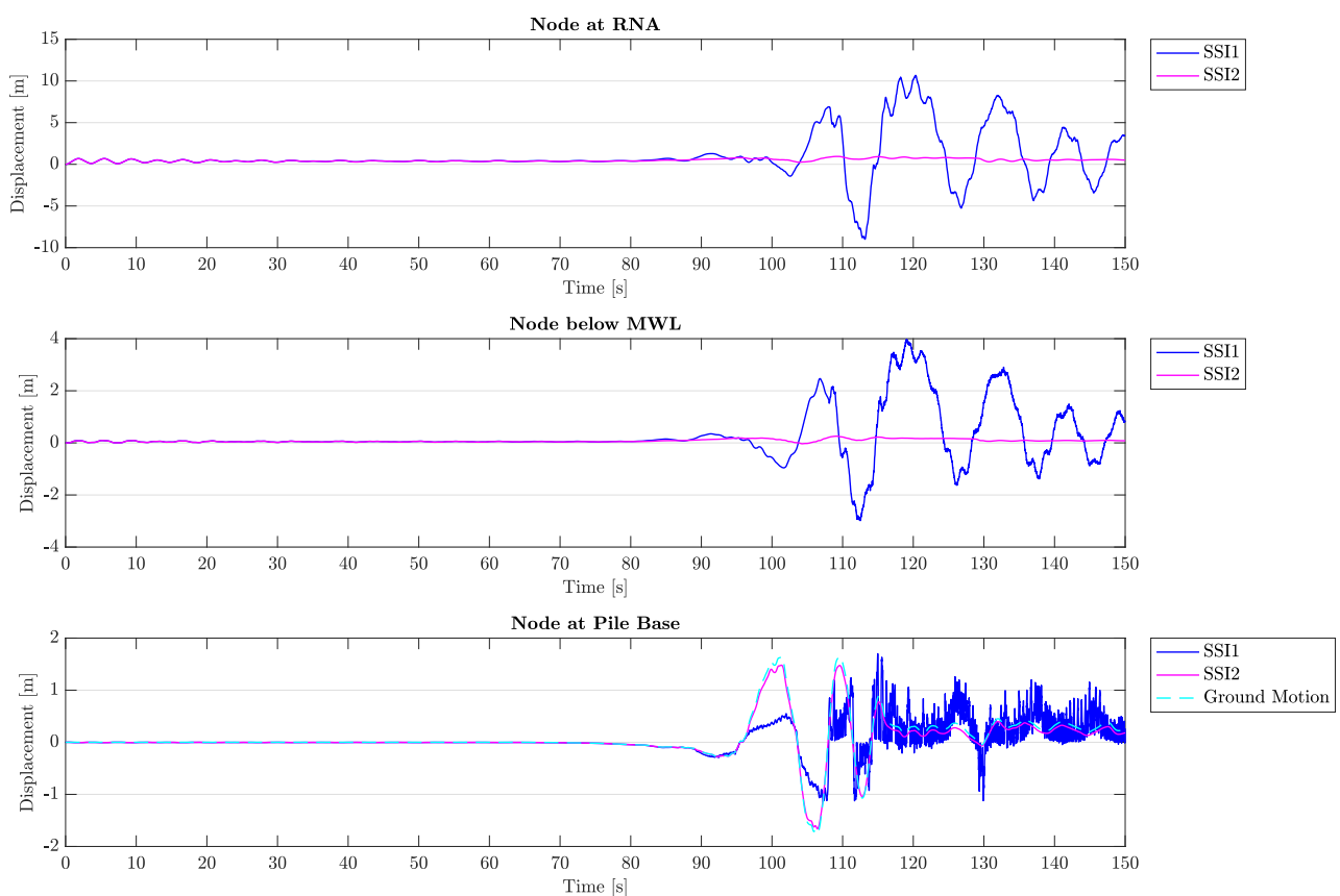
Figure 5.60: Lateral pile displacement time history for SS11 and the simplified SS12 models, for co-directional loading by wind, waves and the Abnormal Level Earthquake, under operational conditions (DLC 4-N). Time history depicted for the RNA node, the node directly below maximum water level, and the node at the pile base below mudline. As a reference, the ground motion is shown versus the pile displacement below mudline.
