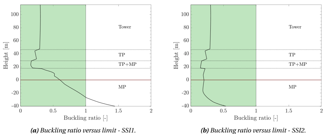
Figure 5.37: Global buckling limit check for the nonlinear elastic soil-structure interaction model (SSII, 5.37a) and the nonlinear inelastic series hysteretic-viscous damping model (SSI2, 5.37b) under wind, wave and earthquake loads, when the turbine is in normal operation mode.
