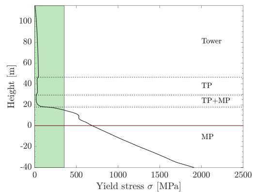
(b) Yield stress versus material yield strength - SSI1.
