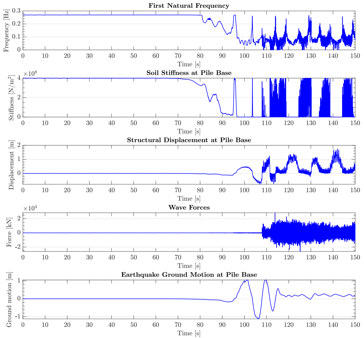
Figure 5.52: Change in first natural frequency over time, in comparison to the change in soil stiffness, change in pile base deflection and wave forcing, for the nonlinear elastic soil-structure interaction model to wind, waves and the Extreme Level Earthquake, after the turbine performed an emergency break.
