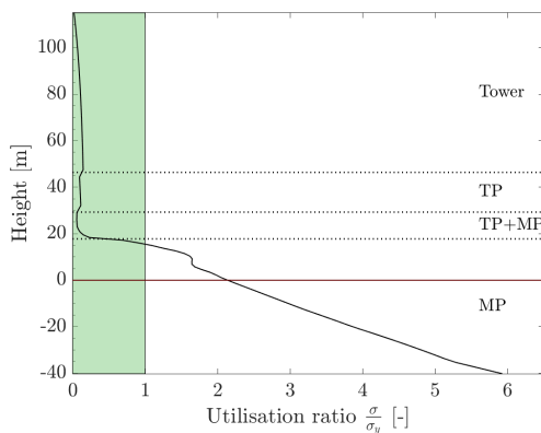
(a) Yield utilization ratio - SSI1.
