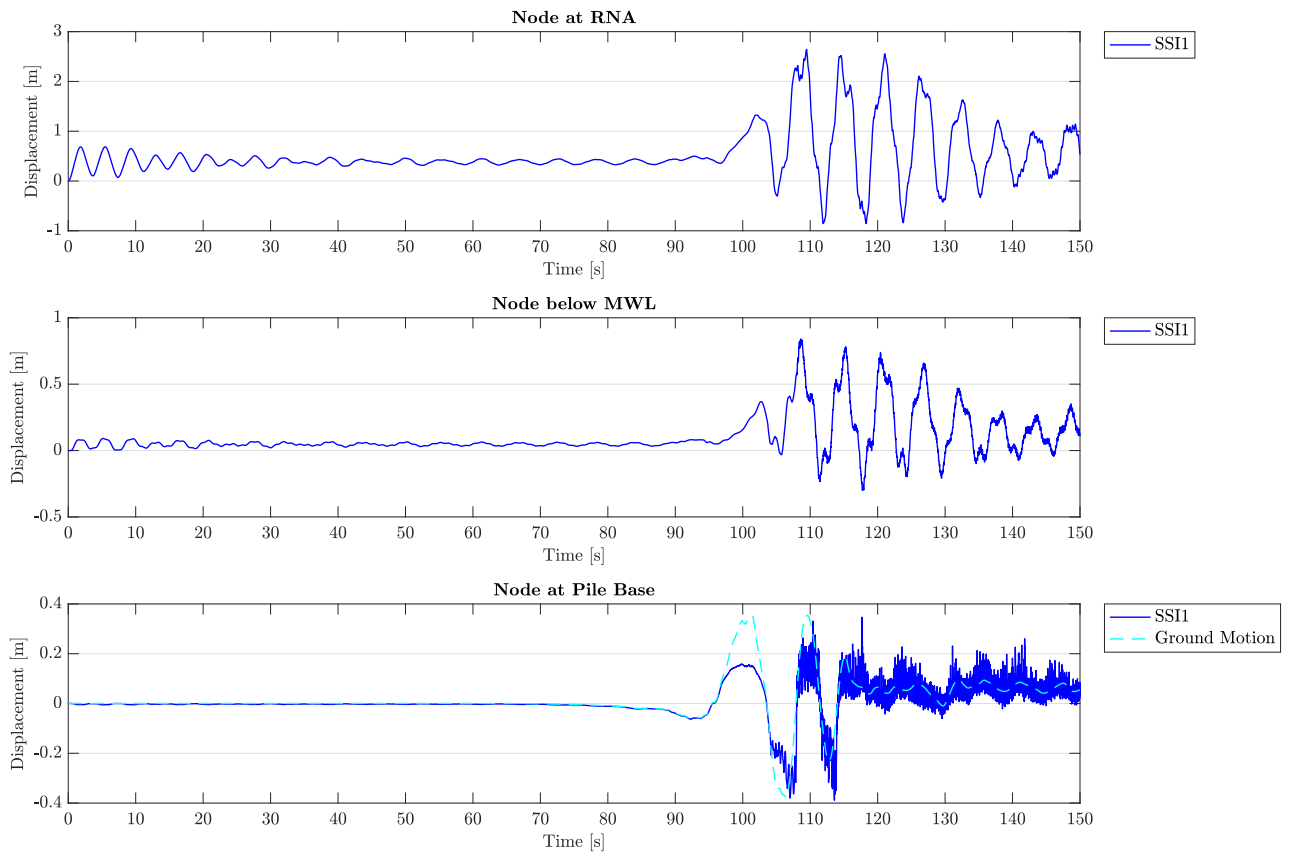
Figure 5.21: Lateral pile displacement time history for the nonlinear elastic soil-structure interaction model (SSl1), for co-directional loading by wind, waves and the recorded earthquake, under operational conditions (DLC 2-N). Time history depicted for the RNA node, the node directly below maximum water level, and the node at the pile base below mudline. As a reference, the ground motion is shown versus the pile displacement below mudline.
