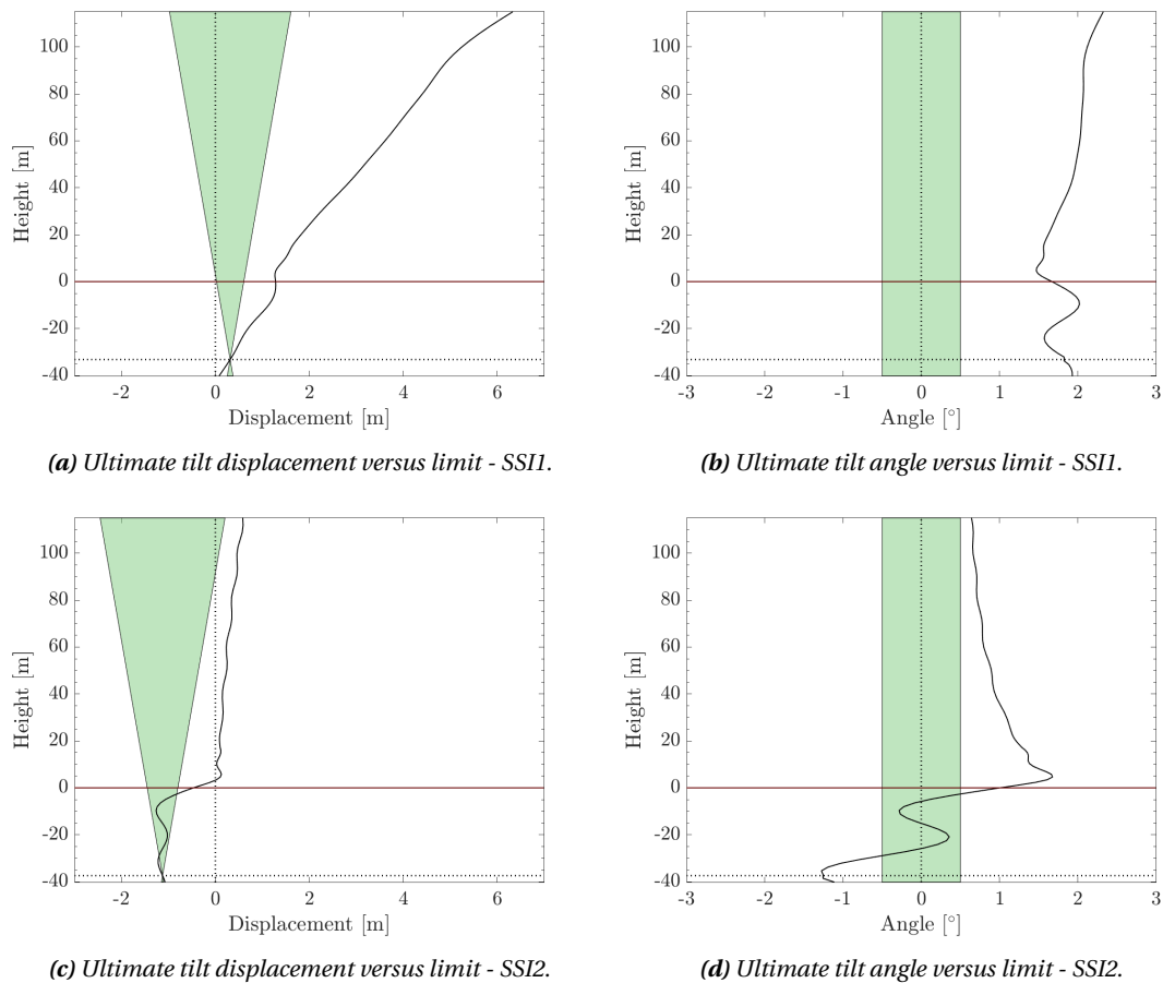
Figure 5.54: Tilt limit check for the nonlinear elastic soil-structure interaction model (SSI1, 5.54a and 5.54b) and the nonlinear inelastic series hysteretic-viscous damping model (SSI2, 5.54c and 5.54d) under wind, wave and Extreme Level Earthquake loads, when the turbine is in normal operation mode.
