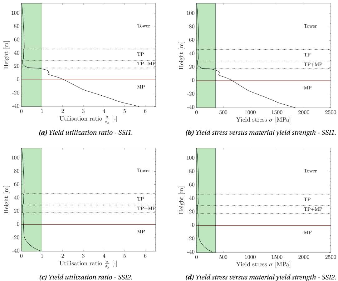
Figure 5.59: Global yield limit check for the nonlinear elastic soil-structure interaction model (SSI1, 5.59a and 5.59b) and the nonlinear inelastic series hysteretic-viscous damping model (SSI2, 5.59c and 5.59d) under wind, wave and Extreme Level Earthquake loads, when the turbine is in emergency shutdown mode.
