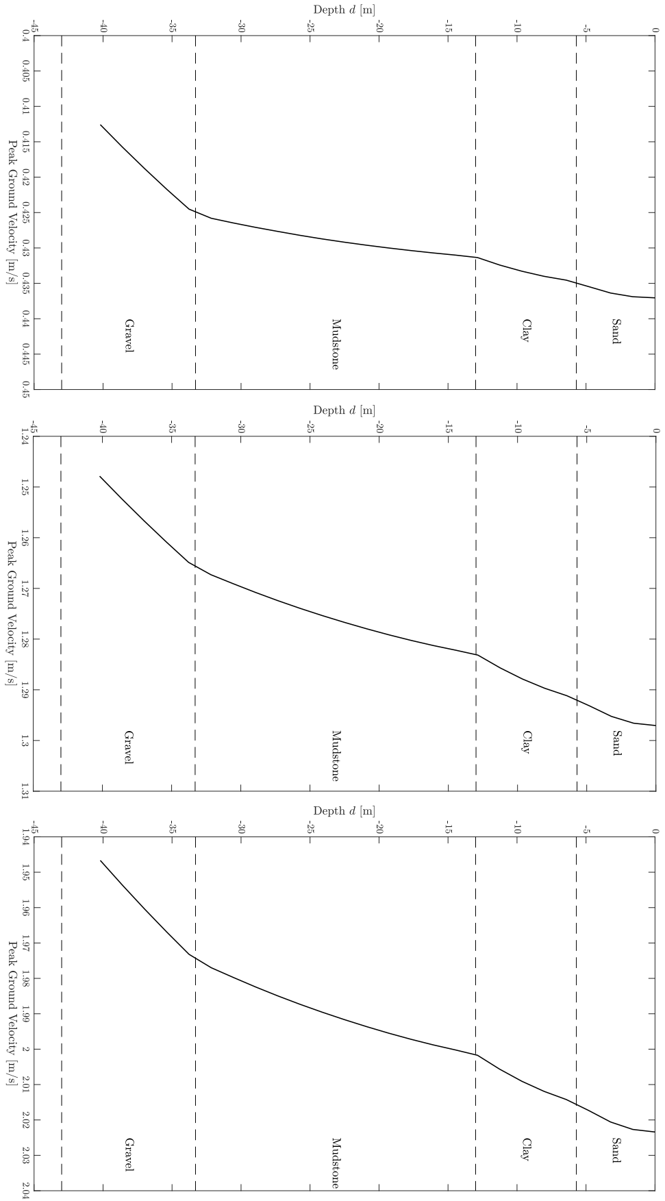
Figure 4.22: Peak ground velocity (PGV) profile from DEEPSOIL linear site response analysis for all IDA levels.
