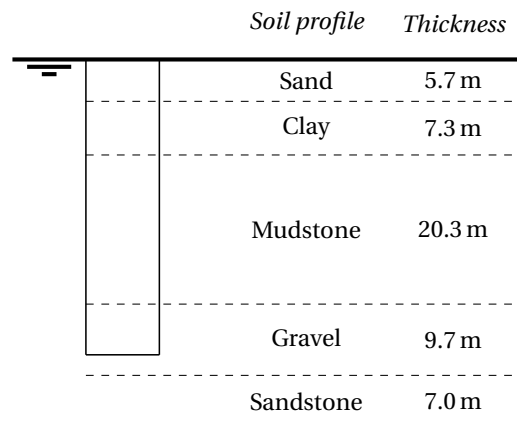
Figure 3.1: Soil profile used in this thesis study.
