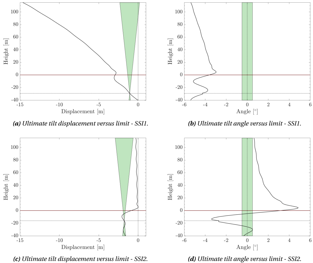
Figure 5.75: Tilt limit check for the nonlinear elastic soil-structure interaction model (SSI1, 5.75a and 5.75b) and the nonlinear inelastic series hysteretic-viscous damping model (SSI2, 5.75c and 5.75d) under wind, wave and Abnormal Level Earthquake loads, after the turbine performed an emergency shutdown.
