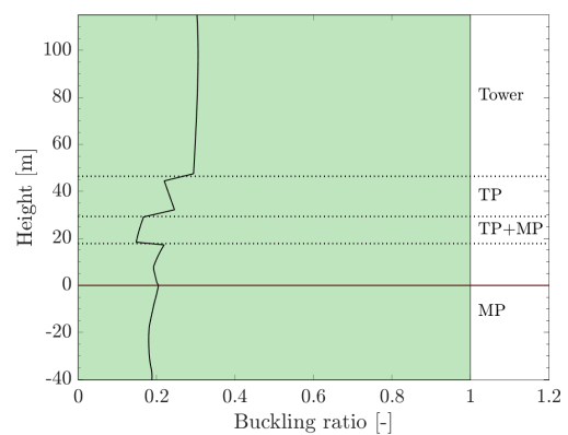
(b) Buckling ratio versus limit - SS12.
