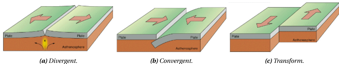
Figure 2.2: Principal types of plate boundaries [76].
