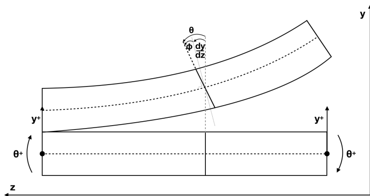
Figure 3.23: Two-node Timoshenko beam element: definition of cross-sectional rotation, shear angle and deflection, and sign convention for the lateral displacement and beam rotation.
