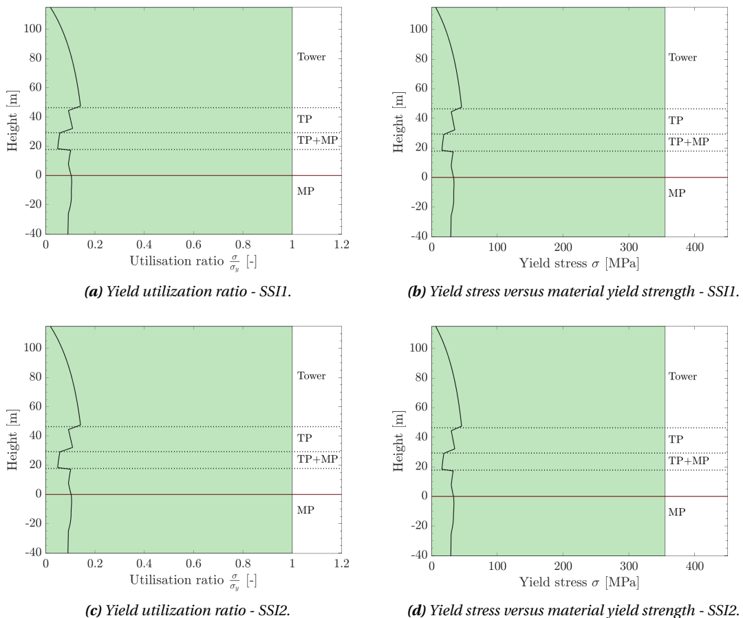
Figure 5.16: Global yield limit check for the nonlinear elastic soil-structure interaction model (SSI1, 5.16a and 5.16b) and the nonlinear inelastic series hysteretic-viscous damping model (SSI2, 5.16c and 5.16d) under wind and wave loads only, when the turbine is in normal operation mode.
