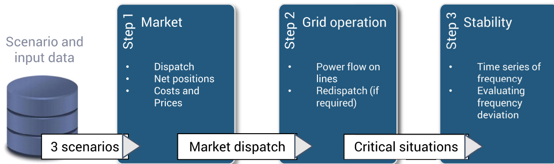
Figure 17: Overview of power system simulation toolchain
