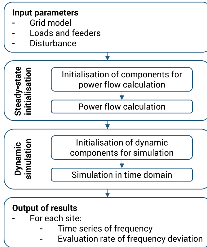
Figure 18: Overview of simulation tool for stability analysis
