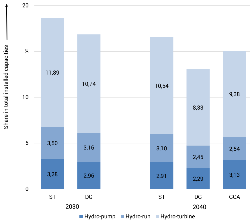
Figure 25: Installed capacities of hydropower, percentage shares of overall installed capacities [104]
