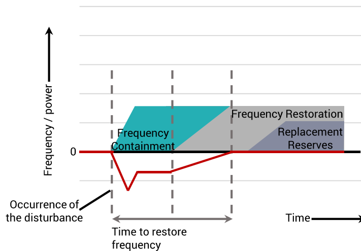
Figure 11: Time frames and measures of regulatory control [47]
