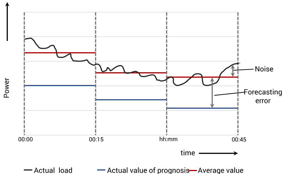
Figure 8: Short-term fluctuations and forecast errors in load
