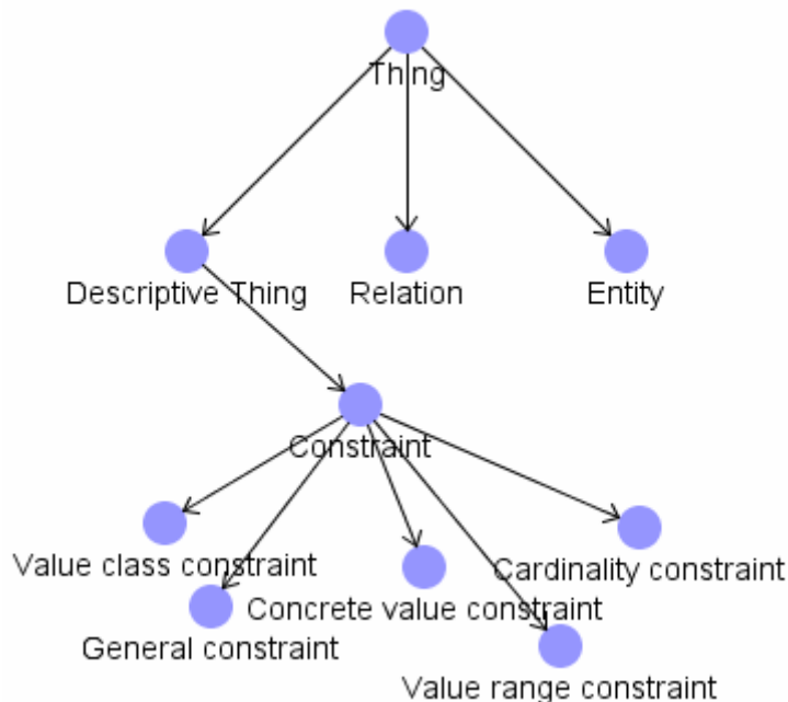
Figure 7.5 - Top ontology
