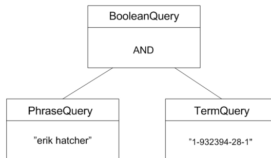
Figure 3.2: Query terms used with appropriate query-methods
