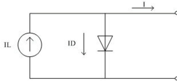
Figur 4.4: Solcelleekvivalentkrets
