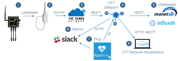
Figure 2: Dataport Protocol Diagram
