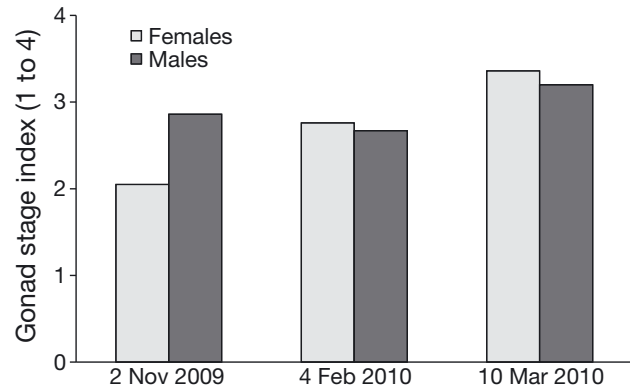
Fig. 3. Gadus morhua . Gonad stage index for Atlantic cod at the Ytterøya farm at different points of time. Gonads: undeveloped (1) to ripe (4)
