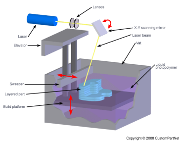
Figure 1.2: SLA
