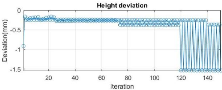
Figure 5.9: Graph of height deviation for experiment (300-1-2).1
