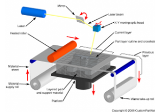
Figure 1.5: Sheet lamination
