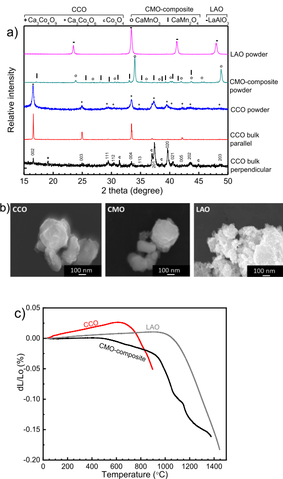
Figure 1. (a) XRD patterns of CCO, CMO-composite, and LAO powders as well as a sample of CCO made by SPS in the directions parallel and perpendicular to the pressing direction, (b) SEM micrographs, and (c) sintering curves of CCO, CMO-composite, and LAO powders produced by spray pyrolysis. Diffraction lines from articles, LAO, 25 CCO, 26 and CMO-composite powder ( \text{CaMnO}_3 27 and \text{CaMn}_2\text{O}_4 28 ) are indicated in (a).
