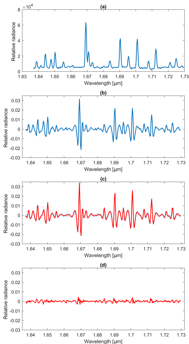
Figure 3. (a) Unfiltered spectrum of the (5, 3) transition. (b) Filtered spectrum of the (5, 3) transition. (c) Normalized spectrum from (b) (blue crosses) with the fitted, filtered model spectrum shown in red. The fitted rotational temperature is 186.5 \pm 0.7 K. (d) Residuals of the fit from (c).
