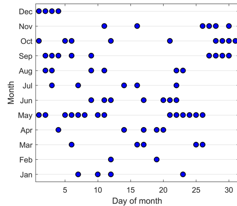
Figure 6. Dates between November 2007 and June 2016 (which is the coverage in the NOTCam archive) when the NOTCam was mounted at the NOT and making spectroscopic astronomical observations.
