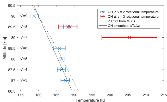
Figure 5. The temperatures from the data presented in Fig. 4 with \Delta v = 2 in blue and \Delta v = 3 in red. Both are presented with their 1\sigma error bar. The altitude of the (9, 7) transition was fixed with a steady-state model using a neutral atmosphere. The altitudes of the other transitions are fixed with a relative distance between neighbouring transitions of 0.5 km, following von Savigny et al. (2012). The NRLMSISE temperature gradient for 19 February 2013 at La Palma ( 17^\circ 53' W , 28^\circ 45' N ) at 05:50 UT is shown as a dashed black line. The same gradient but smoothed with a modelled OH distribution in altitude is shown as a solid black line.
